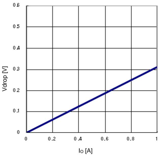
Fig.25 Minimum dropout Voltage 5 (V CC =10V, T a =25°C)
