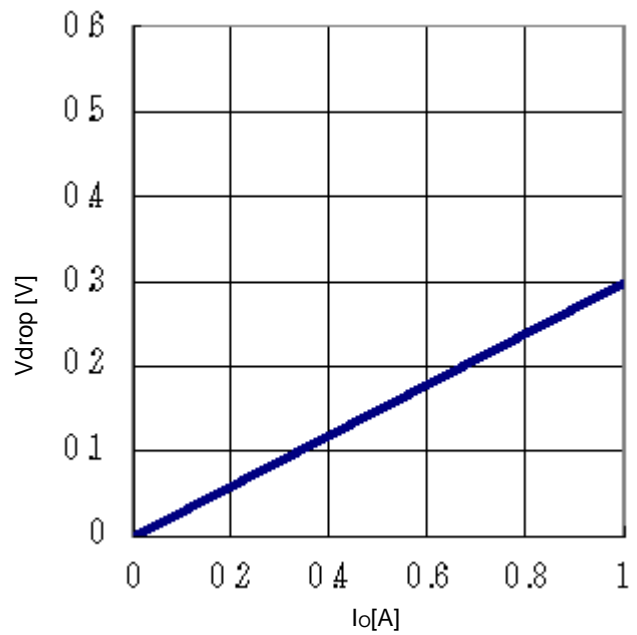
Fig.26 Minimum dropout Voltage 6 (V CC =12V, T a =25°C)
