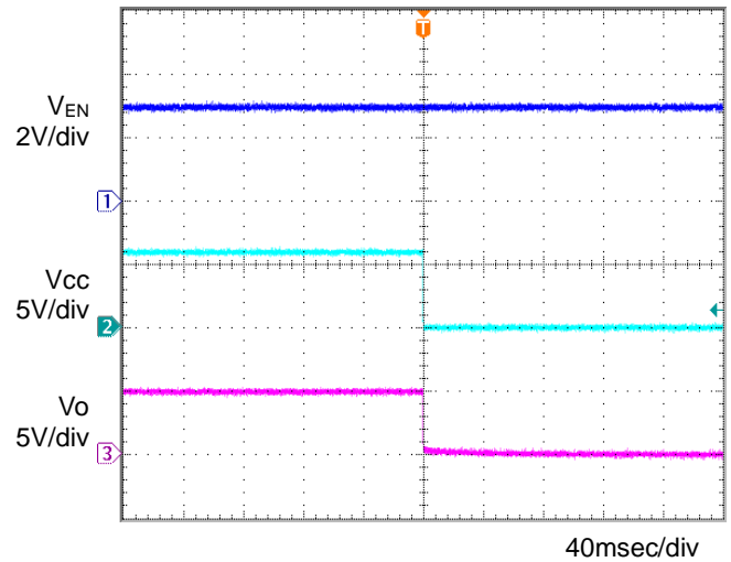
Fig.14 OFF sequence 1 Co=1μF,Ta=125°C
