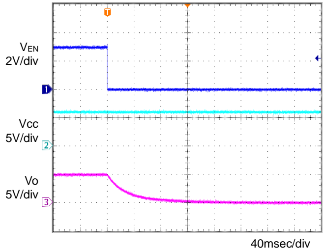
Fig.20 OFF sequence 2 Co=1μF, Ta=125°C
