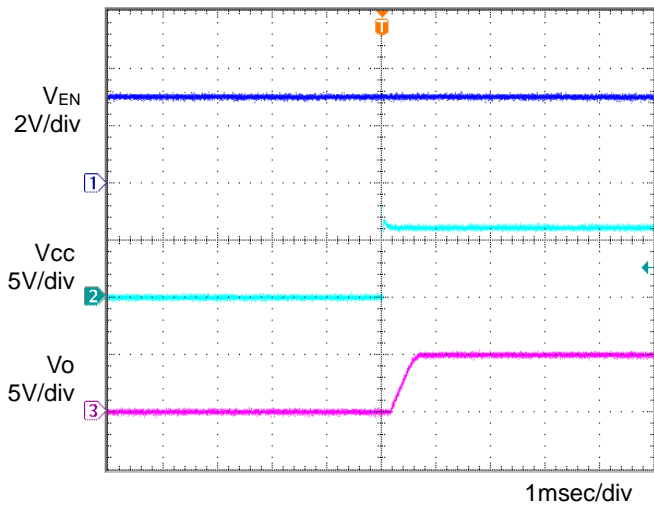
Fig.11 Input sequence 1 Co=1μF,Ta=125°C
