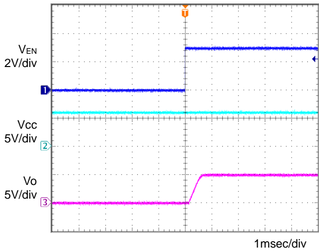
Fig.17 Input sequence 2 Co=1μF, Ta=125°C
