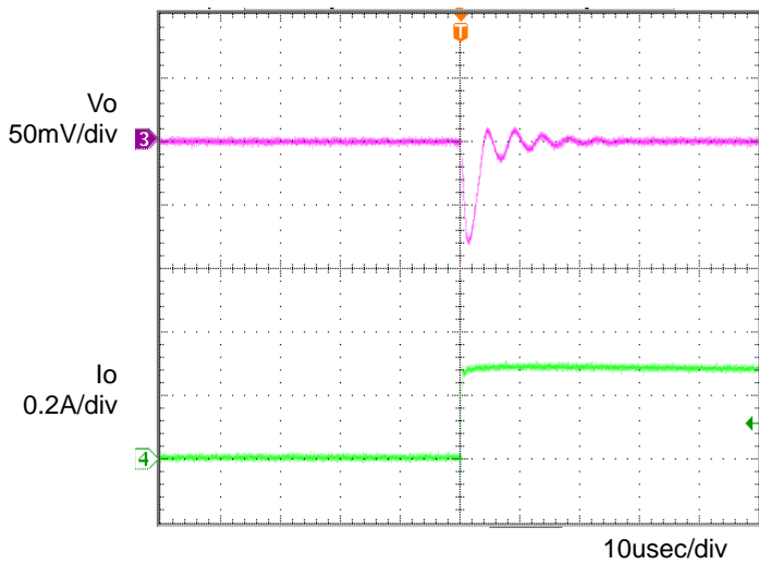
Fig.5 Transient Response (0→0.3A) Co=1μF, Ta=125°C
