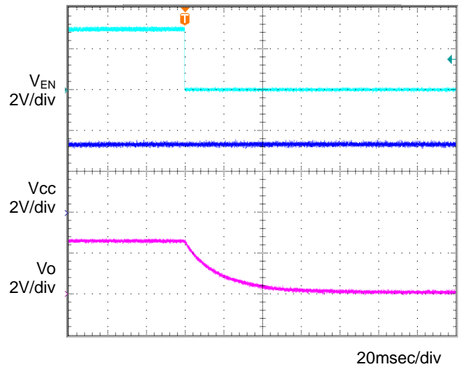
Figure 18. OFF sequence 2 C o =1μF, T a =-40°C
