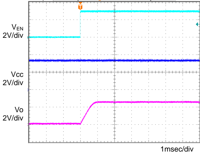
Figure 17. Input sequence 2 C o =1μF, T a =105°C
