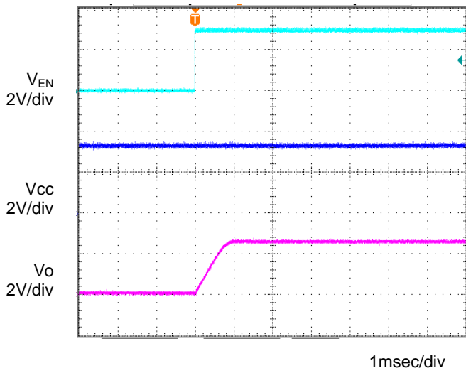
Figure 15. Input sequence 2 C o =1μF, T a =-40°C
