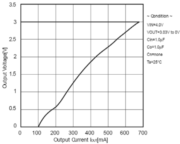
Figure 5. OCP Threshold
