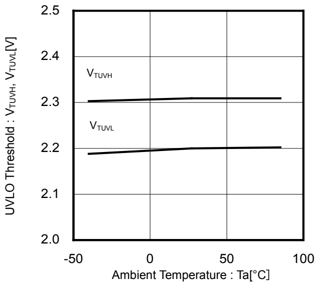
Figure 26. UVLO Threshold Voltage vs Ambient Temperature
