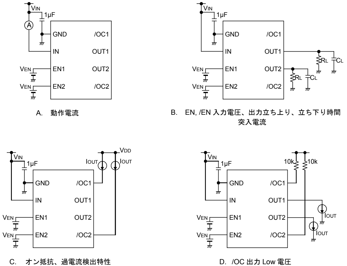
Figure 1. 測定回路
