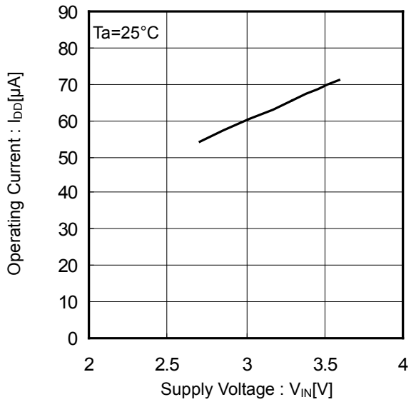
Figure 4. Operating Current vs Supply Voltage (EN Enable)
