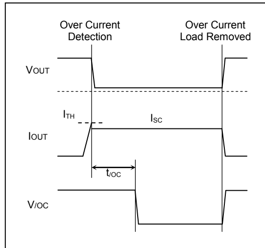
Figure 41. 過電流制限
