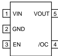
Figure 3. 端子配置 (TOP VIEW)
