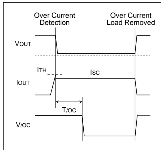
Figure 42. 過電流制限
