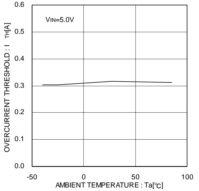
Figure 15. 過電流検出値
