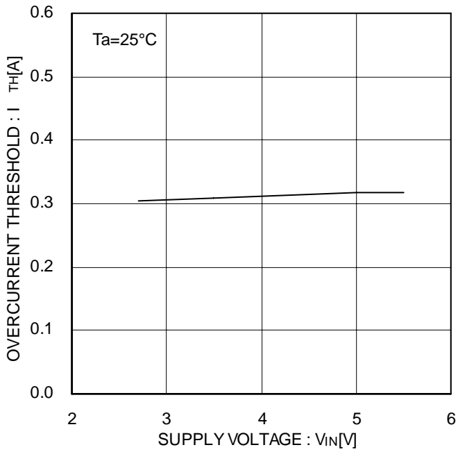
Figure 14. 過電流検出値
