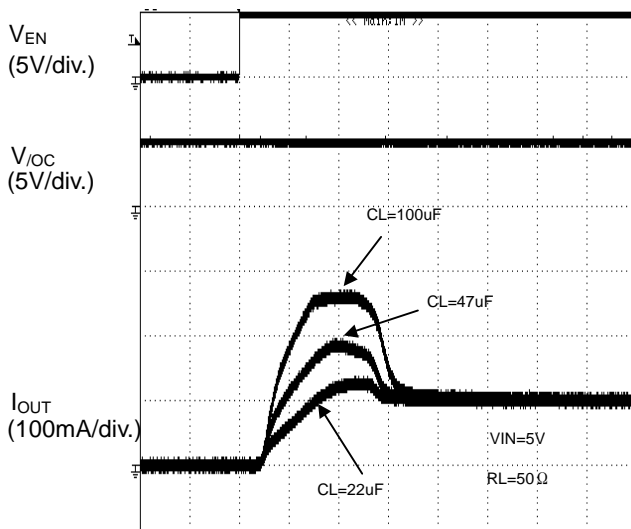
TIME (1ms/div.) Figure 56. 突入電流特性
