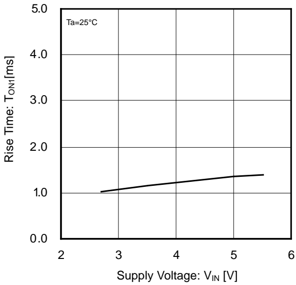
Figure 46. Output rise time vs Suuply Voltage
