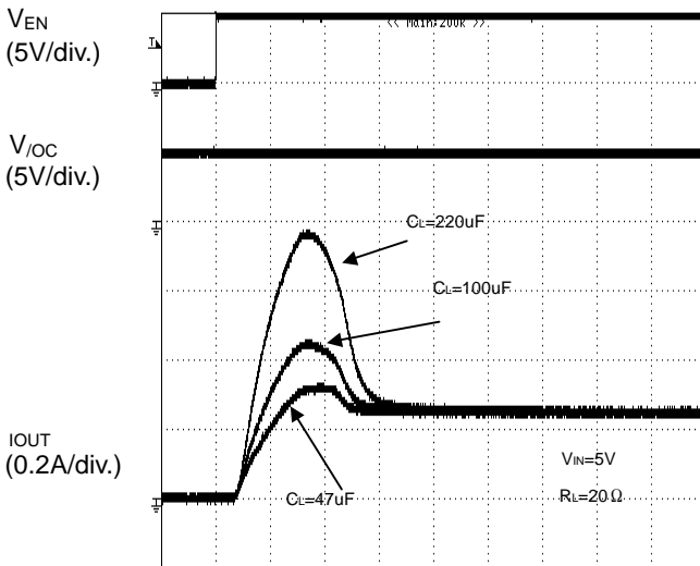
TIME (1ms/div.) Figure 74. 突入電流特性
