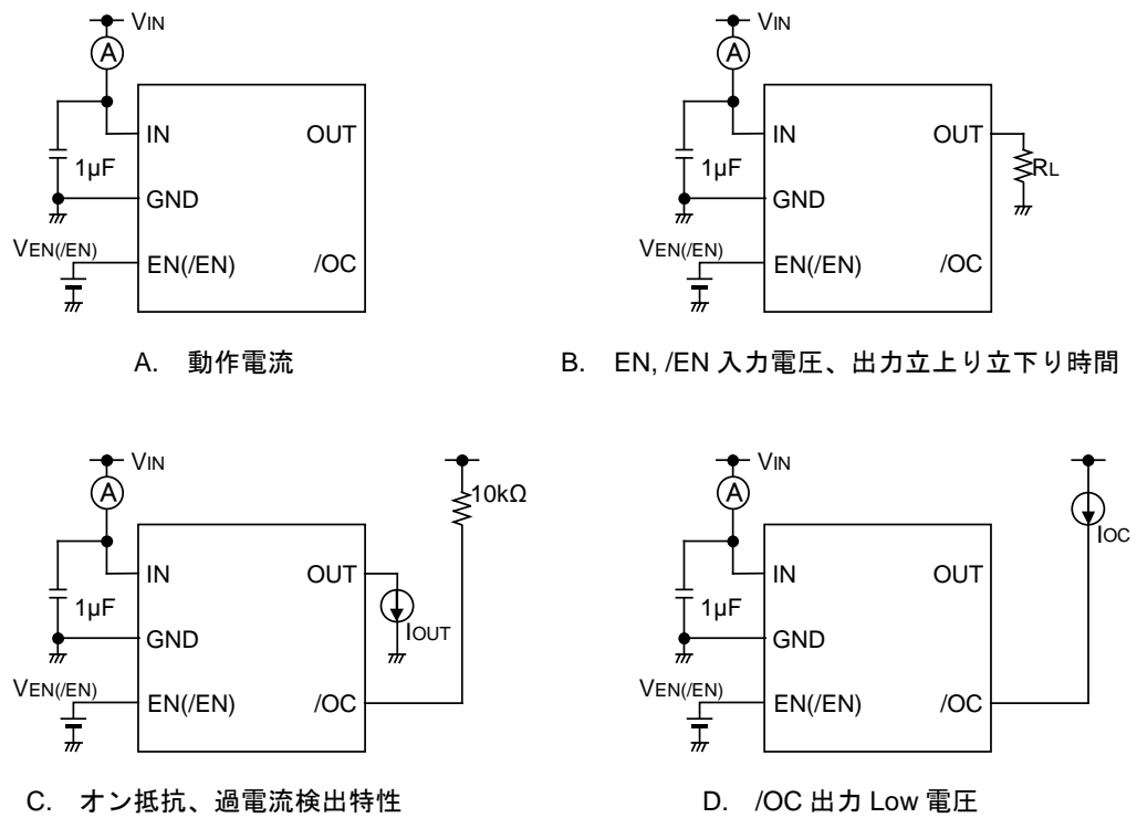
Figure 1. 測定回路
