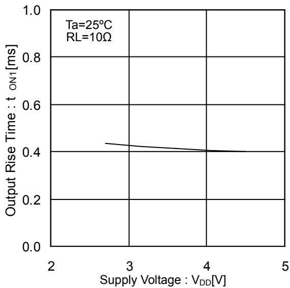
Figure 15. Output Rise Time vs Supply Voltage
