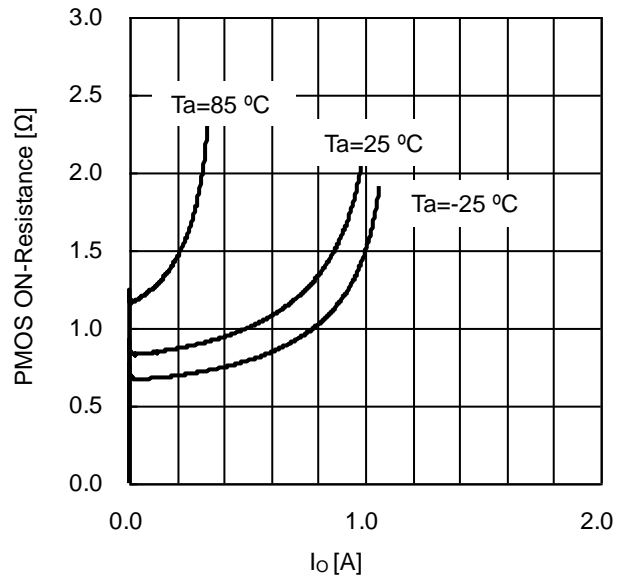
Figure 15. Pch FET ON-Resistance vs Io (VCC=3.5V)
