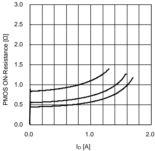
Figure 18. Pch FET ON-Resistance vs I o (V CC =5.0V)
