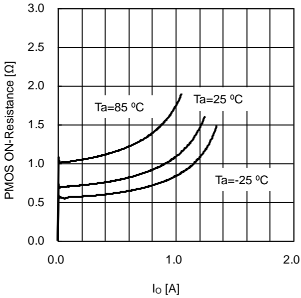
Figure 16. Pch FET ON-Resistance vs I o (V CC =4.0V)
