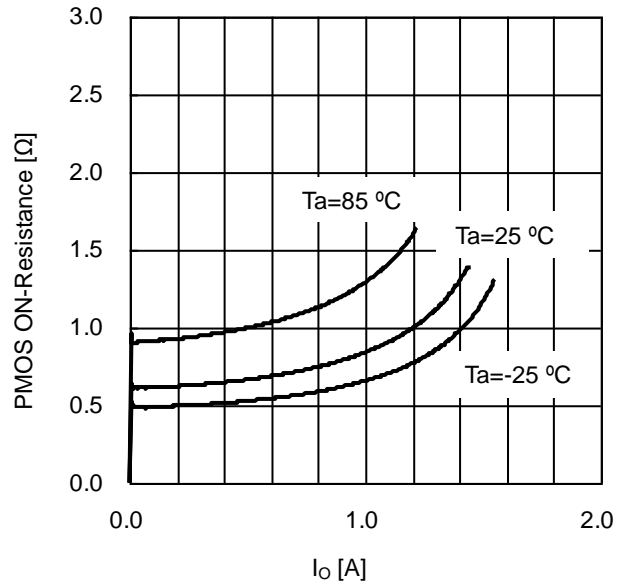
Figure 17. Pch FET ON-Resistance vs I o (V CC =4.5V)
