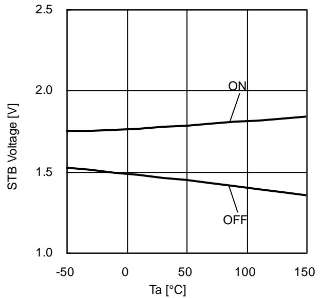
Figure 19. STB Threshold vs Temperature
