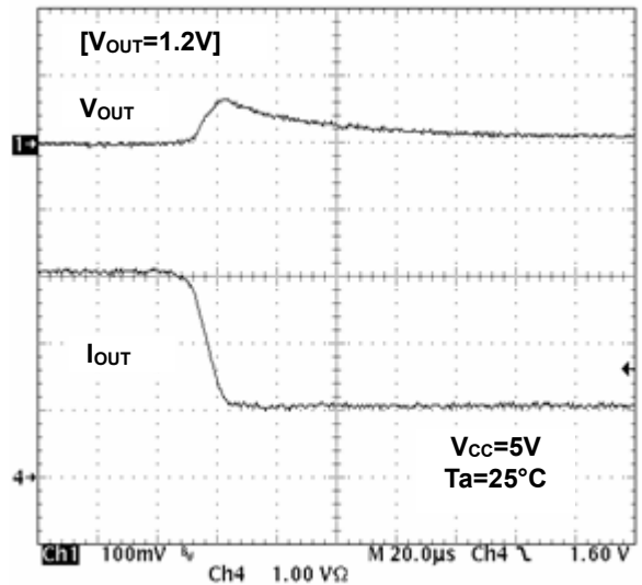
Figure 17. Transient Response (Io=3A~1A, 10µs)
