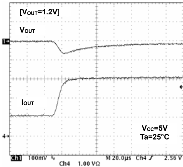
Figure 16. Transient Response (Io=1A~3A, 10µs)
