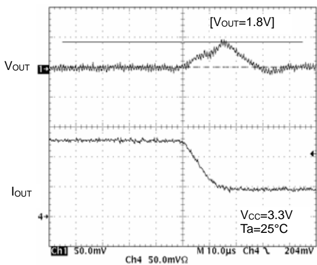
Figure 18. Transient Response (Io=125mA~50mA, 10µs)
