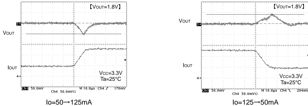
Figure 24. 過渡応答
