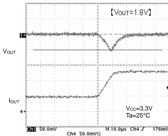
Figure 17. Transient Response (Io=50mA~125mA, 10µs)
