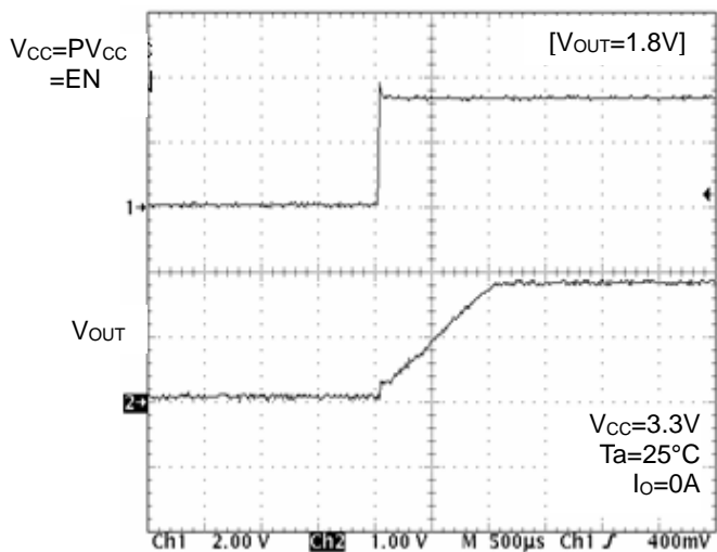
Figure 14. Soft Start Waveform
