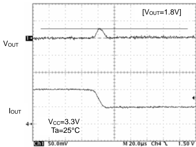
Figure 18. Transient Response ( I_o=2\text{A}\sim 1\text{A}, 10\mu\text{s} )
