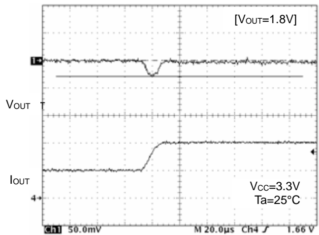
Figure 17. Transient Response ( I_o=1\text{A}\sim 2\text{A}, 10\mu\text{s} )
