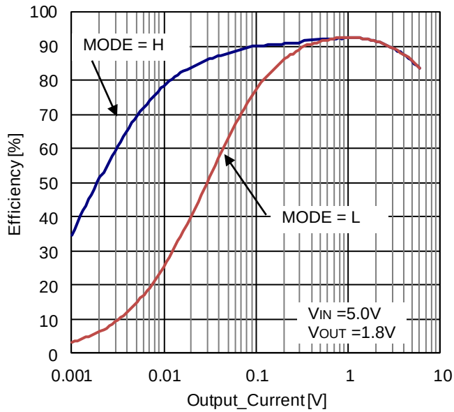
Figure 22. 効率 vs 負荷電流 ( V_{IN} = 5V , V_{OUT} = 1.8V , L = 1.5\mu H )
