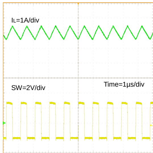
Figure 35. SW 波形 ( V_{IN} = 5.0V , V_{OUT} = 1.8V , I_{OUT} = 6A , L = 1.5\mu H )
