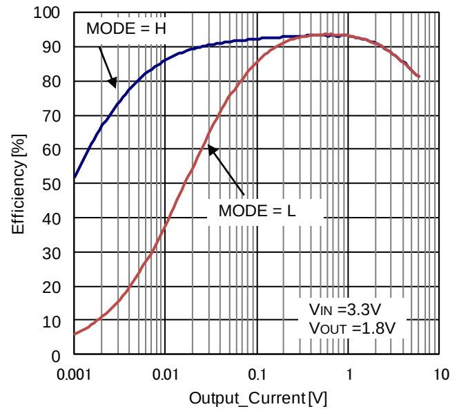
Figure 23. 効率 vs 負荷電流 ( V_{IN} = 3.3V , V_{OUT} = 1.8V , L = 1.0\mu H )
