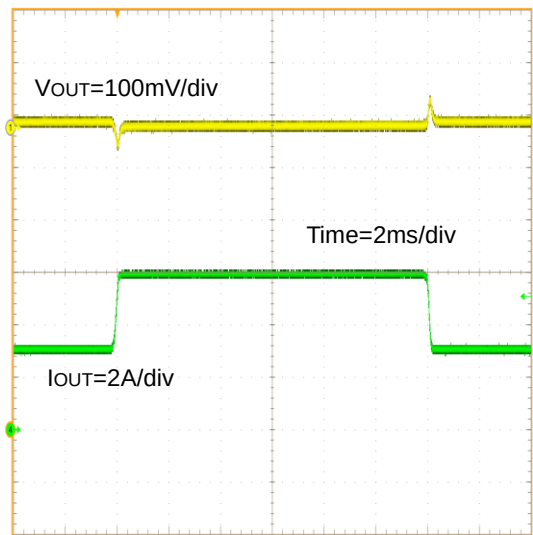
Figure 39. 負荷応答波形 IOUT=3A-6A (VIN=5V, VOUT=1.8V, L=1.5μH, R3=6.8kΩ, C6=5600pF, C14=100pF)
