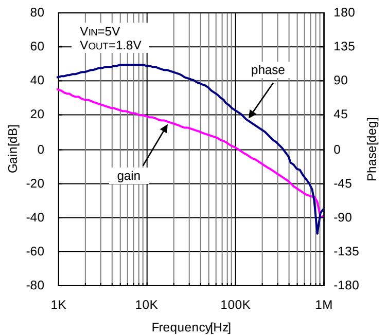
Figure 25. 位相特性 ( V_{IN} = 5V , V_{OUT} = 1.8V , I_{OUT} = 6A , L = 1.5\mu H , R3 = 6.8k\Omega , C6 = 5600pF , C14 = 100pF )
