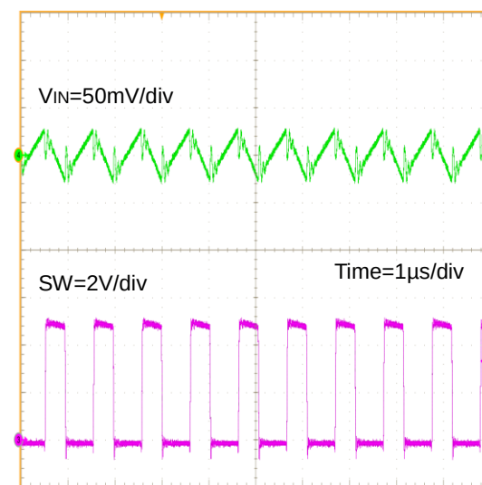
Figure 33. 入力リップル波形 ( V_{IN} = 5V , V_{OUT} = 1.8V , I_{OUT} = 6A )
