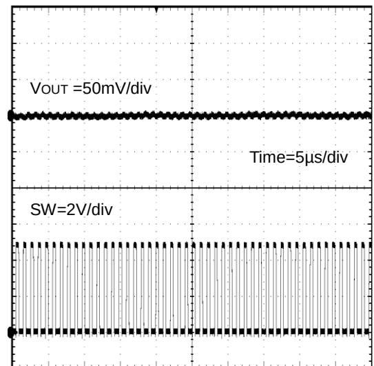
Figure 43. PWM 制御時 SW 波形 ( V_{IN} = 5.0\text{V} , V_{OUT} = 1.8\text{V} , I_{OUT} = 1\text{A} )
