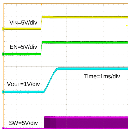
Figure 26. 起動波形 (VIN = EN)
