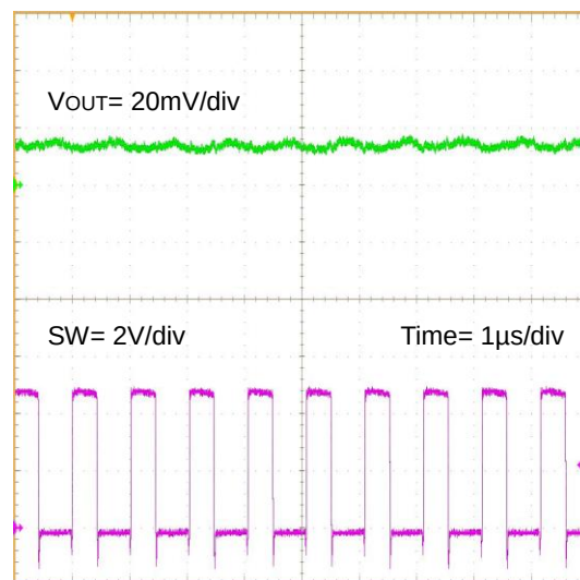
Figure 31. 出力リップル波形 ( V_{IN} = 5V , V_{OUT} = 1.8V , I_{OUT} = 6A )
