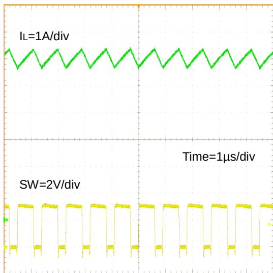
Figure 34. SW 波形 ( V_{IN} = 3.3V , V_{OUT} = 1.8V , I_{OUT} = 6A , L = 1.0\mu H )
