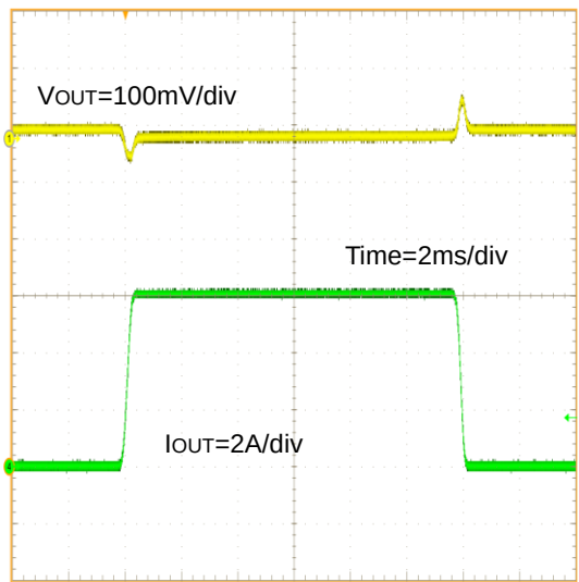
Figure 40. 負荷応答波形 IOUT=0A-6A (VIN=5V, VOUT=1.8V, L=1.5μH, R3=6.8kΩ, C6=5600pF, C14=100pF)
