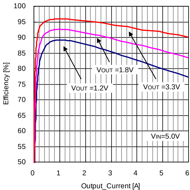
Figure 24. 効率 vs 負荷電流 ( V_{IN} = 5.0V , MODE = 5.0V )
