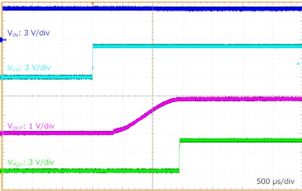
Figure 58. R_{Load} = 0.6\ \Omega EN 起動波形 ( V_{IN} = 5.0\text{ V} , V_{OUT} = 1.8\text{ V} , V_{EN} = 0\text{ V to }5\text{ V} )
