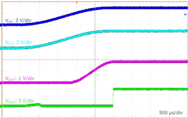
Figure 62. R_{Load} = 0.45\text{ }\Omega VIN 起動波形 ( V_{IN} = V_{EN} = 0\text{ V} to 5\text{ V} , V_{OUT} = 1.8\text{ V} )
