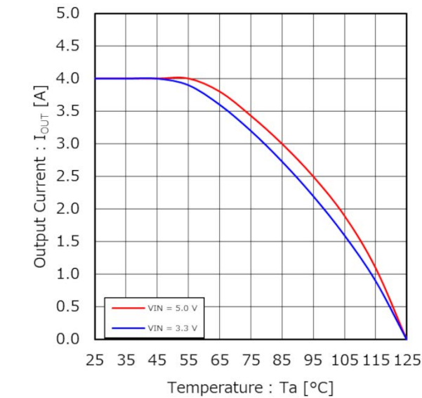
Figure 68. Thermal Derating ( V_{OUT} = 1.8 V)
