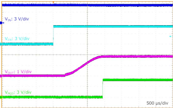
Figure 58. R_{Load} = 0.45\ \Omega EN 起動波形 ( V_{IN} = 5.0\text{ V} , V_{OUT} = 1.8\text{ V} , V_{EN} = 0\text{ V to } 5\text{ V} )
