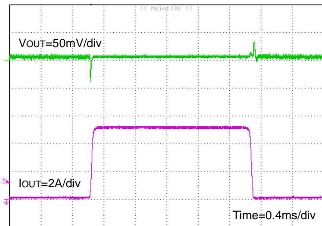
Figure 38. 負荷応答波形 I_{OUT}=0.1A - 5A ( V_{IN}=5V , V_{OUT}=1.2V , FREQ=L , MODE=L , C_{OUT}=\text{Ceramic } 44\mu F )
