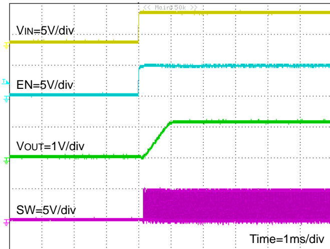
Figure 30. VIN 起動波形 (FREQ=H, RLOAD=0.2Ω)
