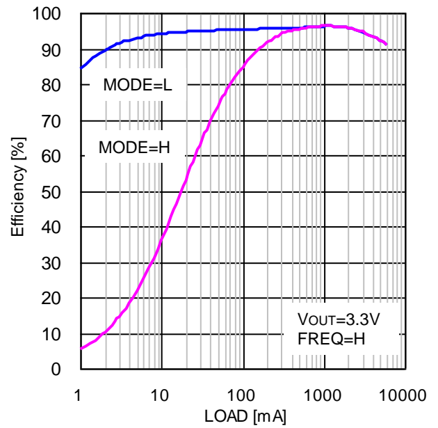
Figure 9. 効率 vs 負荷電流 (VIN=5V, VOUT=3.3V, L=1.0 \mu H, FREQ=H)
