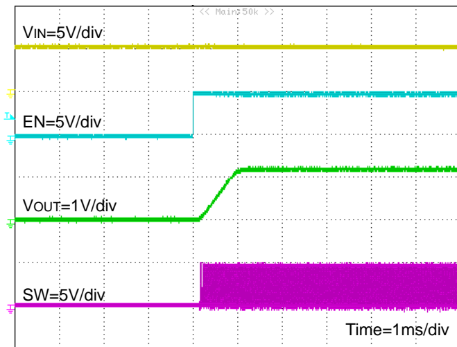
Figure 28. EN 起動波形 (FREQ=H, RLOAD=0.2Ω)
