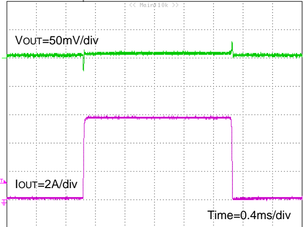
Figure 39. 負荷応答波形 I_{OUT}=0.1A - 6A ( V_{IN}=5V , V_{OUT}=1.2V , FREQ=L , MODE=H , C_{OUT}=\text{Ceramic } 44\mu F )
