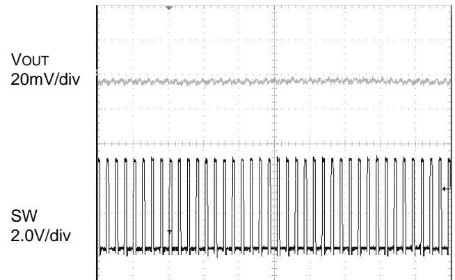
Figure 42. PWM 制御時 SW 波形) ( V_{IN} = 5.0V , V_{OUT} = 1.2V , I_{OUT} = 6A )
