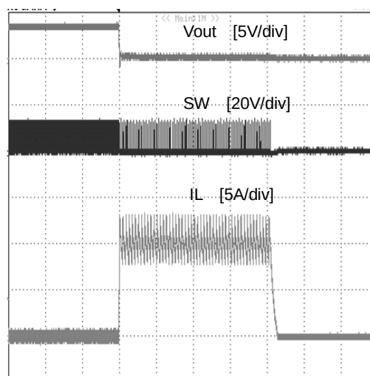
Figure 15. OCP 波形 (Vin=12V, Vout=3.3V, L=4.7μH, Cout=44μF, Vout is short to GND)
