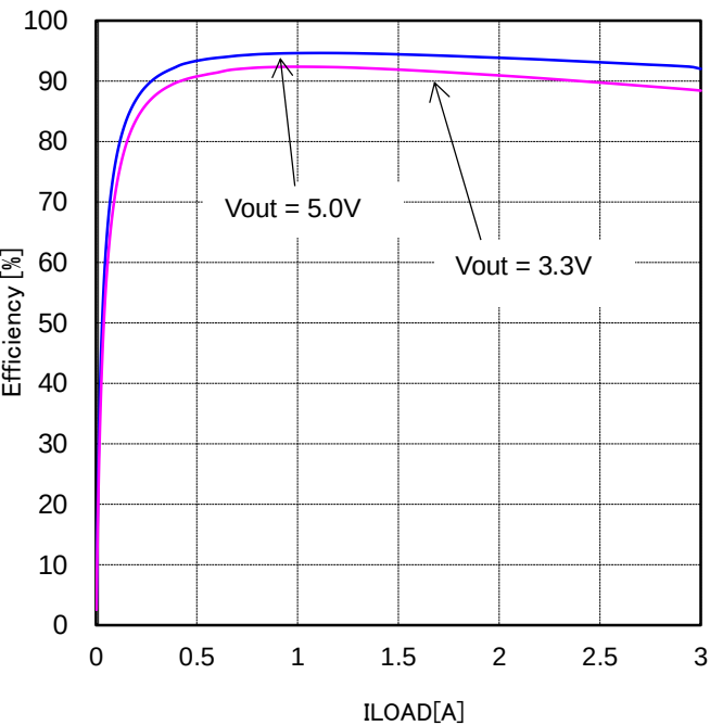
Figure 4. 効率 (VIN=12V, L=4.7μH)
