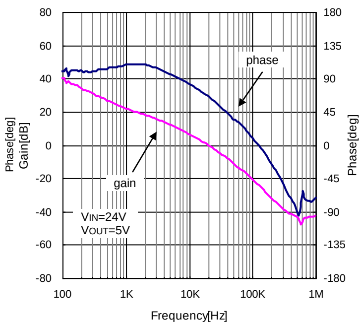
Figure 38. 位相特性 ( V_{IN}=24V , V_{OUT}=5V , I_{OUT}=1.0A , C_{OUT}=\text{Ceramic}22\mu F \times 2 )
