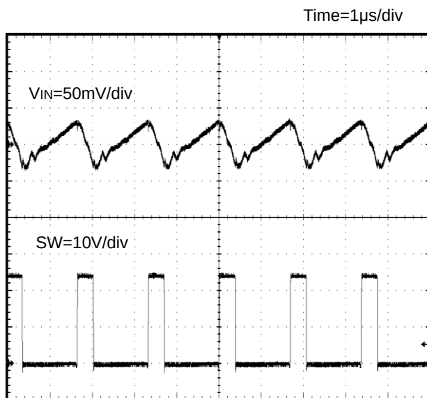
Figure 28. V IN リップル波形 (V IN = 24V, V OUT = 5V, I OUT = 1.0A)
