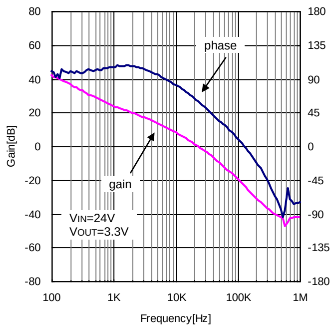
Figure 37. 位相特性 ( V_{IN}=24V , V_{OUT}=3.3V , I_{OUT}=1.0A , C_{OUT}=\text{Ceramic}22\mu F \times 2 )
