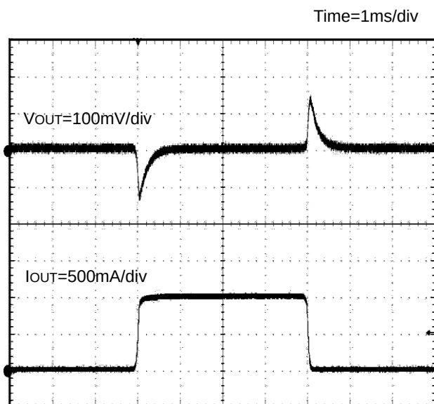
Figure 39. 負荷応答波形 I_{OUT}=0A - 1.0A ( V_{IN}=24V , V_{OUT}=3.3V , C_{OUT}=\text{Ceramic}22\mu F \times 2 )
