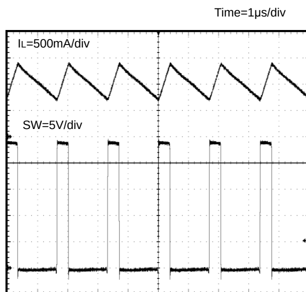
Figure 30. SW 波形 ( V_{IN} = 24\text{V} , V_{OUT} = 5\text{V} , I_{OUT} = 1.0\text{A} )
