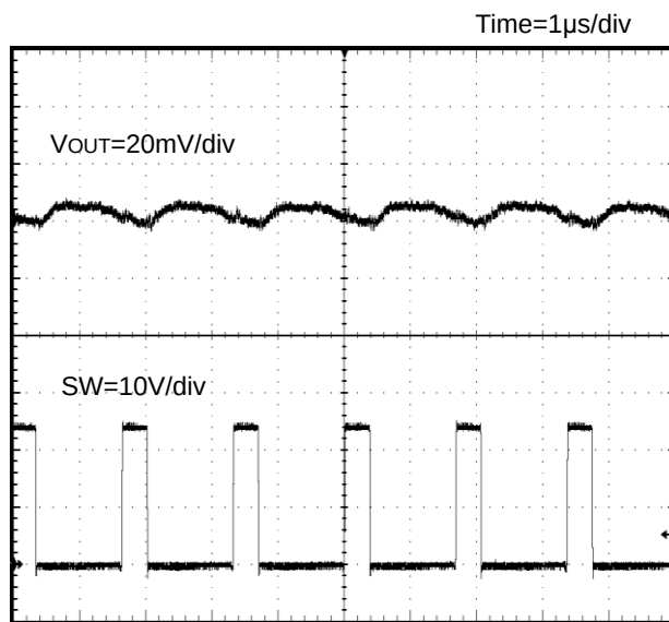
Figure 26. V OUT リップル波形 (V IN = 24V, V OUT = 5V, I OUT = .1.0A)
