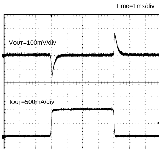
Figure 40. 負荷応答波形 I_{OUT}=0A - 1.0A ( V_{IN}=24V , V_{OUT}=5V , C_{OUT}=\text{Ceramic}22\mu F \times 2 )
