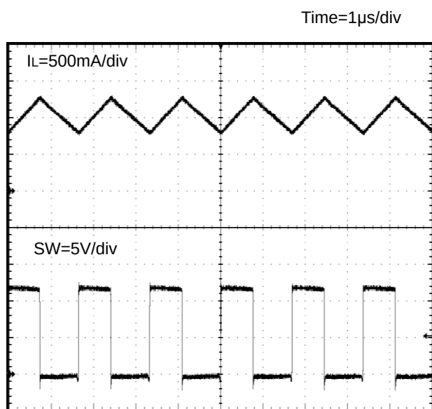
Figure 29. SW 波形 ( V_{IN} = 12\text{V} , V_{OUT} = 5\text{V} , I_{OUT} = 1.0\text{A} )
