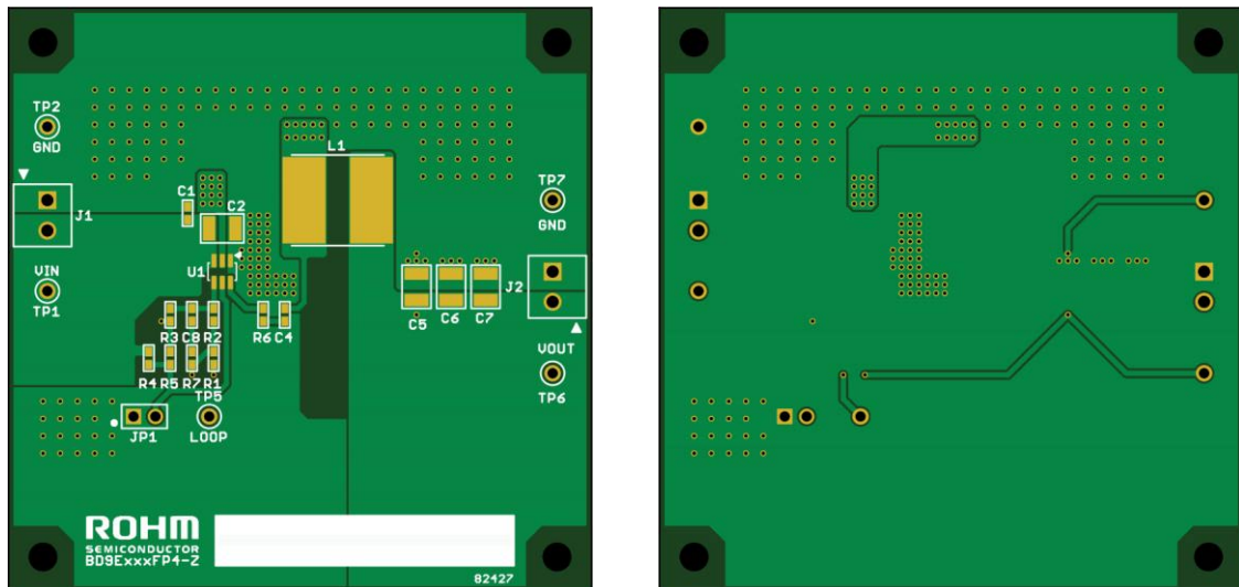
Figure 61. PCB レイアウト例 (Silkscreen Overlay)
