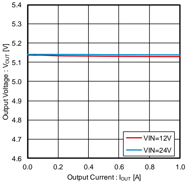
Figure 15. Output Voltage vs Output Current
