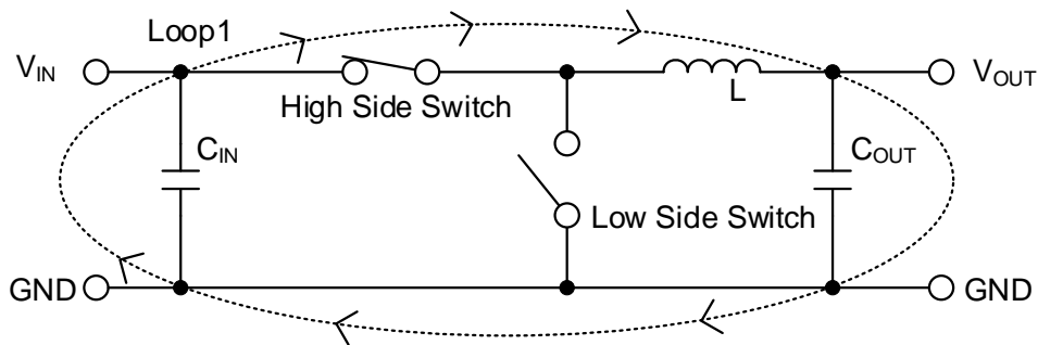
Figure 59-a. High Side Switch = ON, Low Side Switch = OFF 時の電流経路
