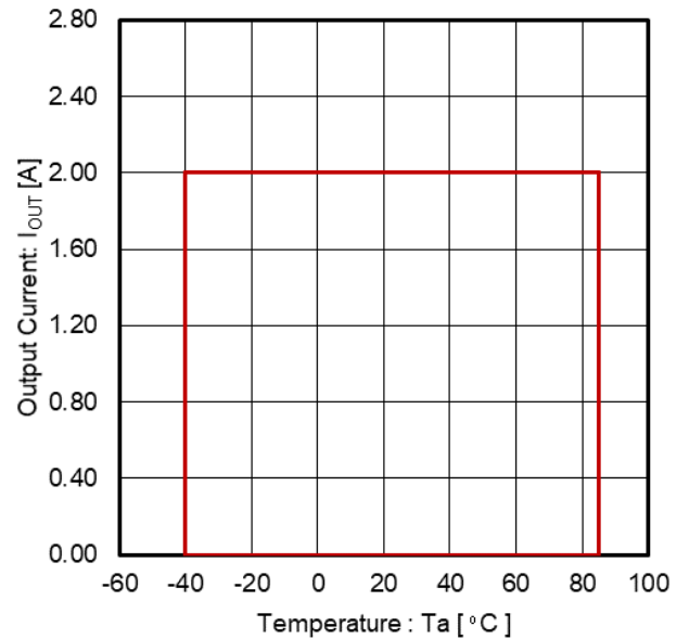
Figure 28. Output Current vs Temperature (Note 1) Operating Range: T_j < 150\text{ }^\circ\text{C} ( V_{IN} = 12\text{ V}, 24\text{ V}, V_{OUT} = 5\text{ V} )
