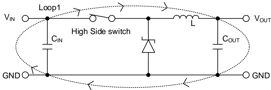
Figure 61-a. High Side switch: ON 時の電流経路
