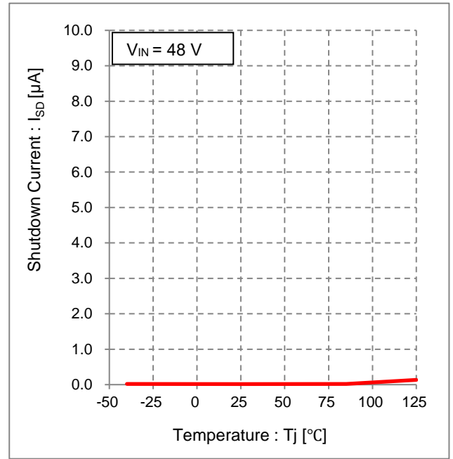
Figure 2. Shutdown Current vs Temperature
