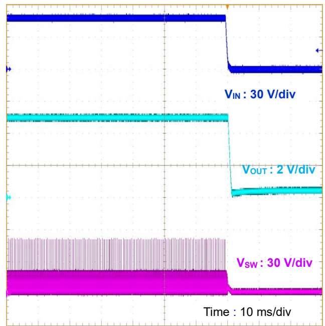
Figure 18. シャットダウン波形 ( V_{IN} = V_{EN} , V_{IN} = 48\text{ V} , V_{OUT} = 5\text{ V} , f_{OSC} = 200\text{ kHz} , I_{OUT} = 0\text{ A} )
