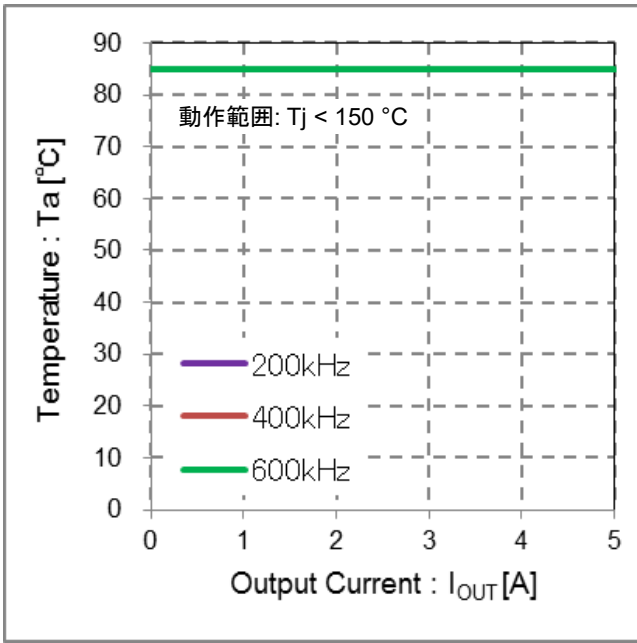
Figure 29. Temperature vs Output Current ( V_{IN} = 48\text{ V} , V_{OUT} = 5\text{ V} , ROHM 評価ボード)
