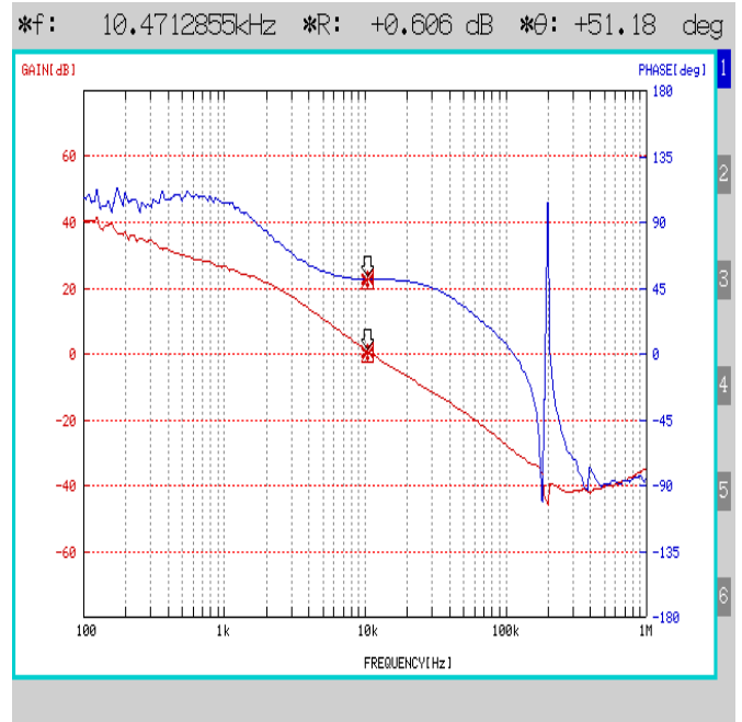
Figure 45. Frequency Characteristics ( I_{OUT} = 5.0\text{ A} )
