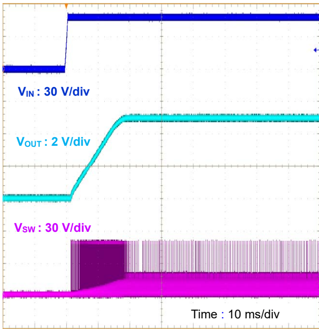
Figure 17. 起動波形 ( V_{IN} = V_{EN} , V_{IN} = 48\text{ V} , V_{OUT} = 5\text{ V} , f_{OSC} = 200\text{ kHz} , I_{OUT} = 0\text{ A} )
