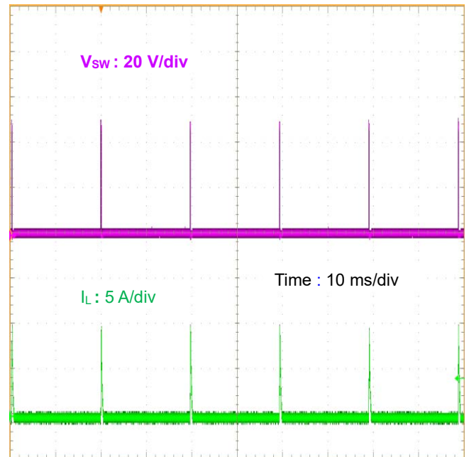
Figure 28. SW 波形 ( V_{IN} = 48\text{ V} , V_{OUT} = 5\text{ V} , f_{OSC} = 200\text{ kHz} , V_{OUT} short to GND)
