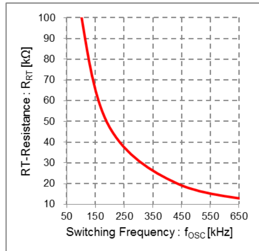
Figure 58. RT-Resistance vs Switching Frequency
