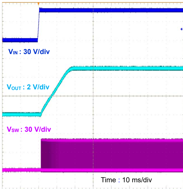
Figure 19. 起動波形 ( V_{IN} = V_{EN} , V_{IN} = 48\text{ V} , V_{OUT} = 5\text{ V} , f_{OSC} = 200\text{ kHz} , I_{OUT} = 5\text{ A} )
