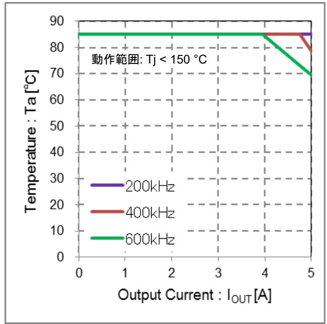
Figure 30. Temperature vs Output Current ( V_{IN} = 48\text{ V} , V_{OUT} = 12\text{ V} , ROHM 評価ボード)
