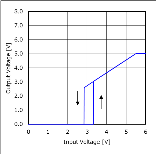
Figure 84. 出力電圧 vs 入力電圧 (R LOAD = 5 Ω)
