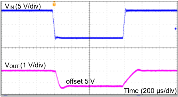
Figure 82. 入力応答 2 (VIN = 16 V to 4 V、I OUT = 1 A)
