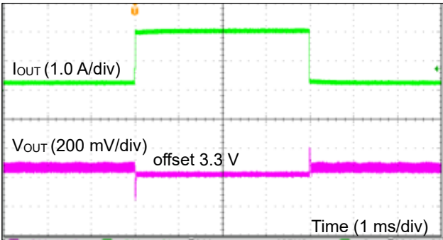
Figure 63. 負荷応答 2 (VIN = 12 V、V MODE = 0 V、I OUT = 0.1 A ~ 1 A)
