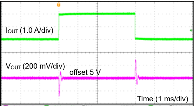
Figure 79. 負荷応答 1 (VIN = 12 V、V MODE = 3.3 V、I OUT = 0 A ~ 1 A)
