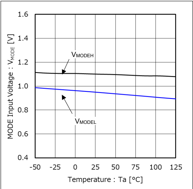
Figure 7. MODE 入力電圧 vs 温度
