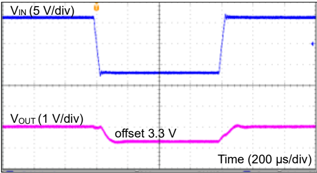
Figure 95. 入力応答 2 (VIN = 16 V to 3 V、I OUT = 1 A)
