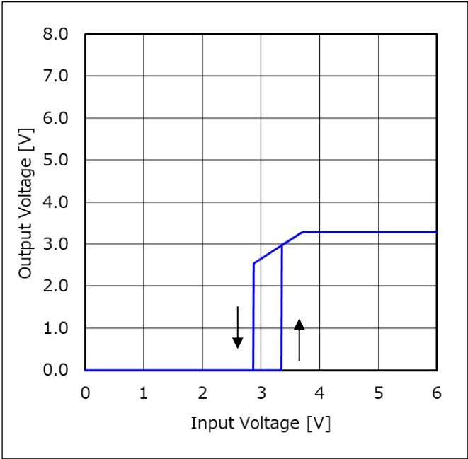
Figure 97. 出力電圧 vs 入力電圧 (R LOAD = 3.3 Ω)
