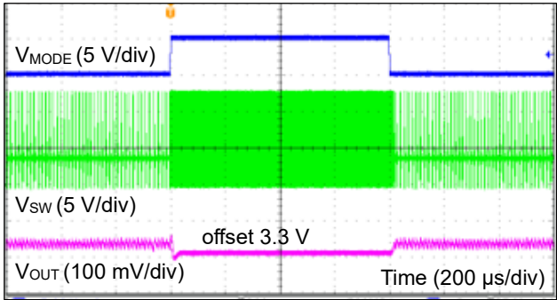
Figure 61. MODE ON/OFF 応答 (VIN = 12 V、IOUT = 50 mA)
