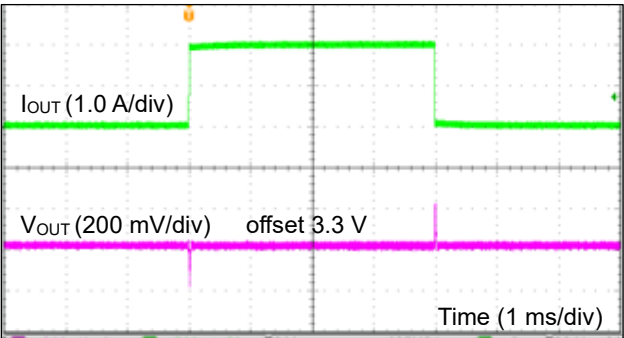
Figure 62. 負荷応答 1 (VIN = 12 V、V MODE = 3.3 V、I OUT = 0 A ~ 1 A)
