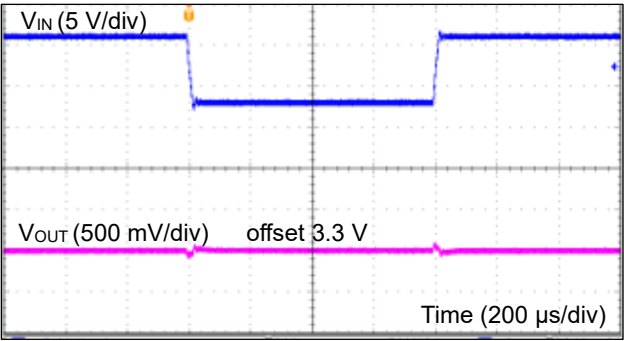
Figure 94. 入力応答 1 (VIN = 16 V to 8 V、I OUT = 1 A)
