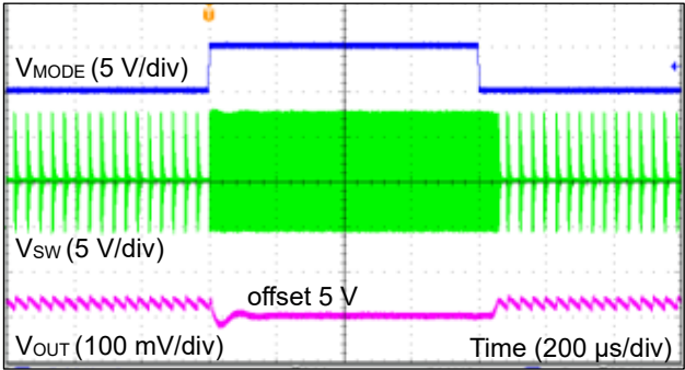
Figure 78. MODE ON/OFF 応答 (VIN = 12 V、IOUT = 50 mA)
