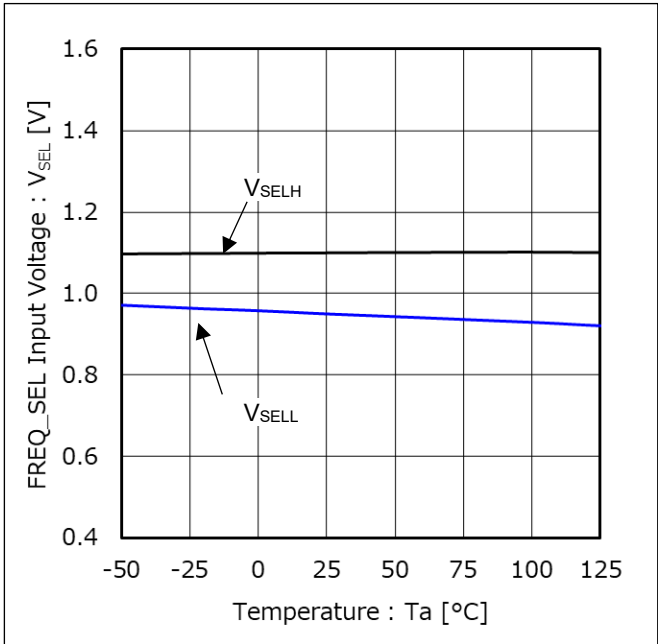
Figure 8. FREQ_SEL 入力電圧 vs 温度
