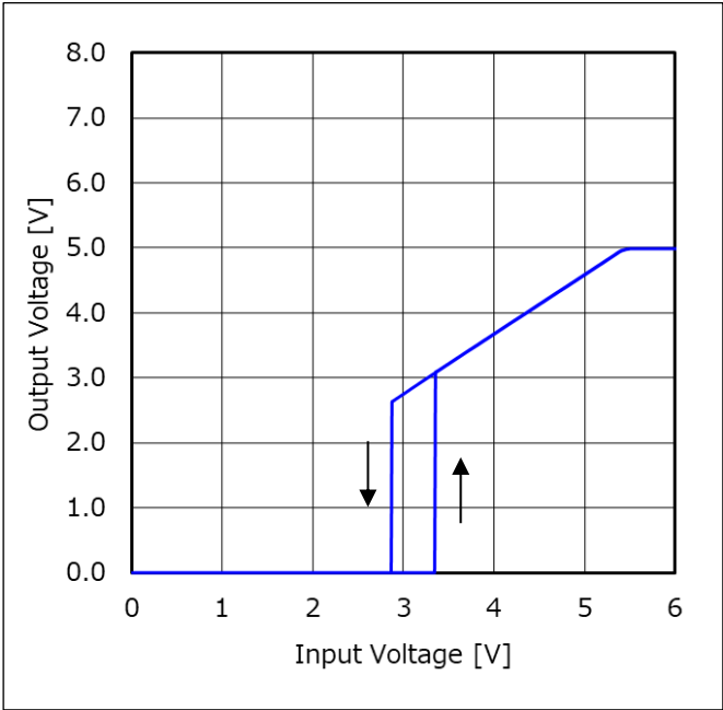
Figure 50. 出力電圧 vs 入力電圧 (R LOAD = 5 Ω)
