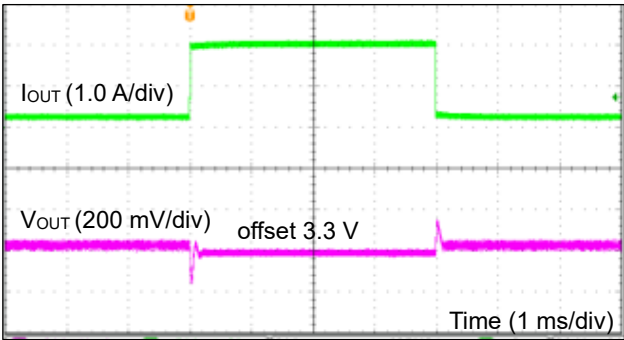
Figure 93. 負荷応答 2 (VIN = 12 V、V MODE = 0 V、I OUT = 0.1 A ~ 1 A)
