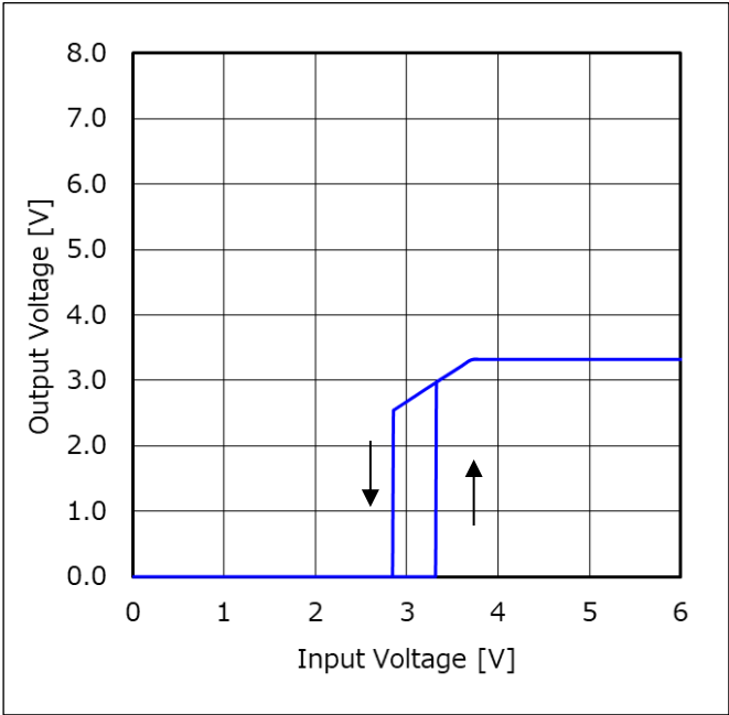
Figure 67. 出力電圧 vs 入力電圧 (R LOAD = 3.3 Ω)
