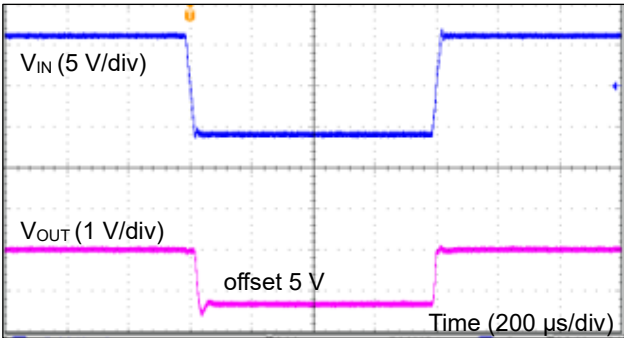
Figure 48. 入力応答 2 (VIN = 16 V ~ 4 V、I OUT = 1 A)
