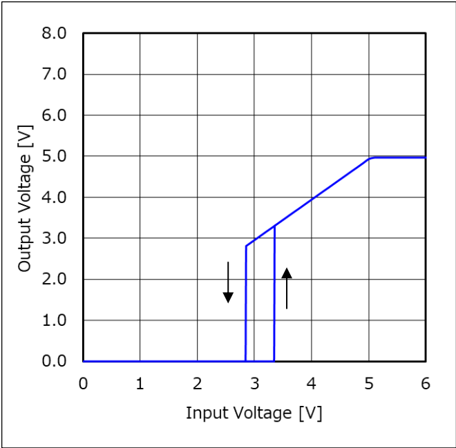
Figure 49. 出力電圧 vs 入力電圧 (R LOAD = 250 Ω)
