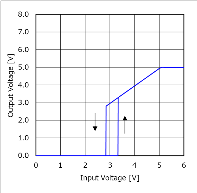
Figure 83. 出力電圧 vs 入力電圧 (R LOAD = 250 Ω)
