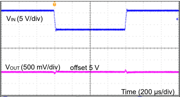
Figure 47. 入力応答 1 (VIN = 16 V ~ 8 V、I OUT = 1 A)
