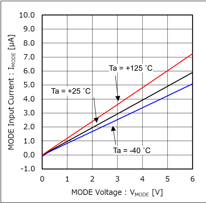
Figure 9. MODE 流入電流 vs MODE 入力電圧
