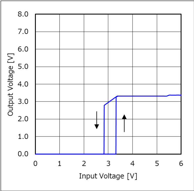
Figure 66. 出力電圧 vs 入力電圧 (R LOAD = 165 Ω)
