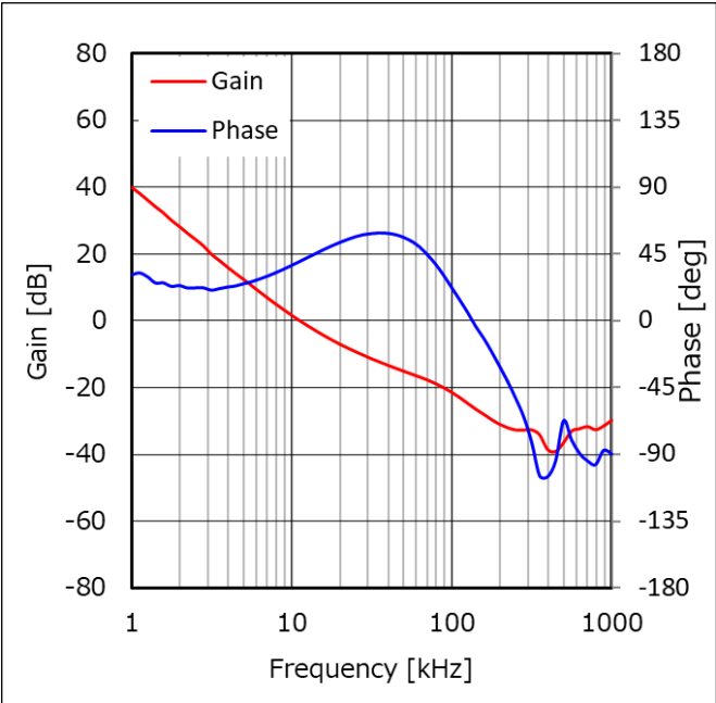
Figure 90. 周波数特性 (VIN = 12 V、IOUT = 0.5 A)
