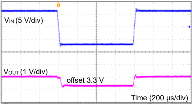
Figure 65. 入力応答 2 (VIN = 16 V to 3 V、I OUT = 1 A)
