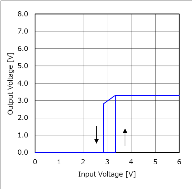
Figure 96. 出力電圧 vs 入力電圧 (R LOAD = 165 Ω)
