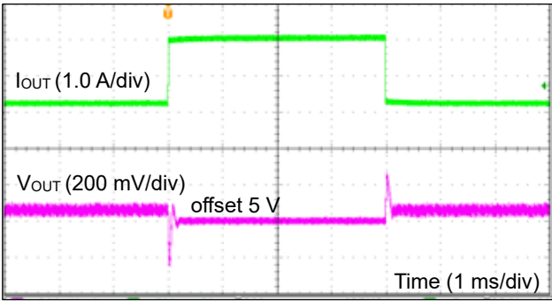
Figure 80. 負荷応答 2 (VIN = 12 V、V MODE = 0 V、I OUT = 0.1 A ~ 1 A)
