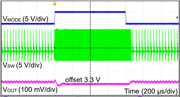
Figure 91. MODE ON/OFF 応答 (VIN = 12 V、IOUT = 50 mA)
