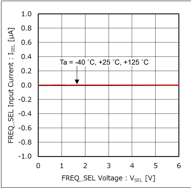
Figure 10. FREQ_SEL 流入電流 vs FREQ_SEL 入力電圧
