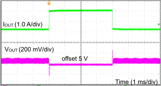
Figure 46. 負荷応答 2 (VIN = 12 V、V MODE = 0 V、I OUT = 0.1 A ~ 1 A)
