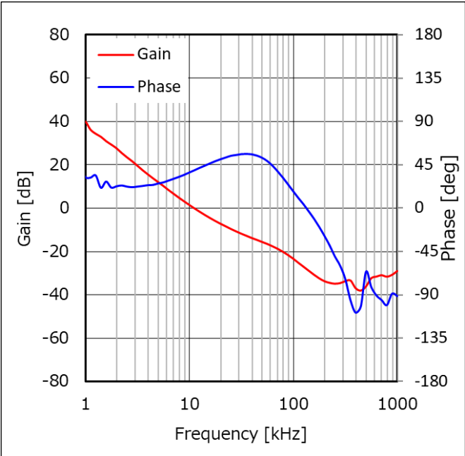
Figure 77. 周波数特性 (VIN = 12 V、IOUT = 0.5 A)
