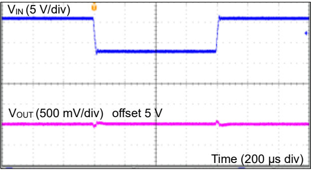
Figure 81. 入力応答 1 (VIN = 16 V to 8 V、I OUT = 1 A)
