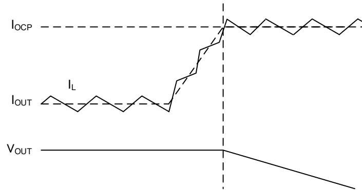
Figure 32. 過電流保護
