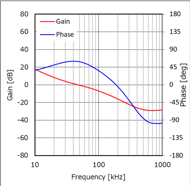
Figure 60. 周波数特性 (VIN = 12 V、IOUT = 0.5 A)
