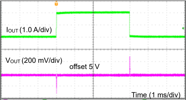
Figure 45. 負荷応答 1 (VIN = 12 V、V MODE = 3.3 V、I OUT = 0 A ~ 1 A)
