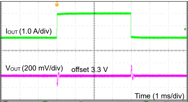
Figure 92. 負荷応答 1 (VIN = 12 V、V MODE = 3.3 V、I OUT = 0 A ~ 1 A)
