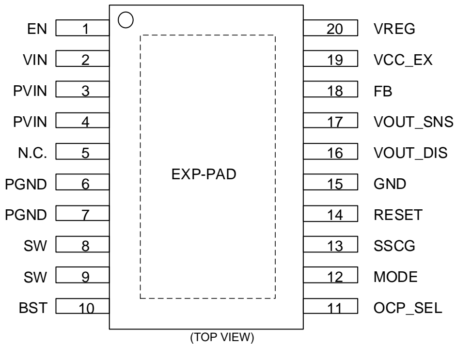
Figure 6. 端子配置図 (BD9P206EFV-C)
