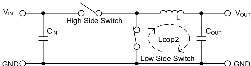
Figure 89 (b). High Side Switch : OFF、Low Side Switch : ON 時の電流経路
