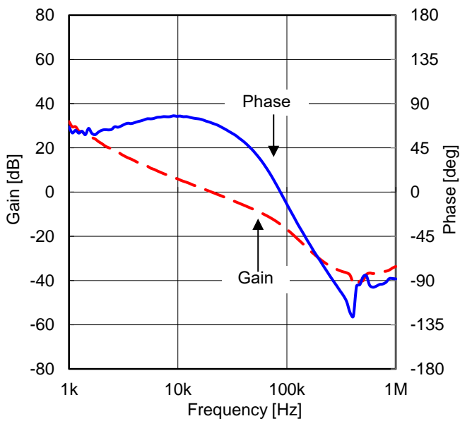
Figure 65. 周波数特性 ( V_{IN} = 12\text{ V} , I_{OUT} = 1.0\text{ A} )
