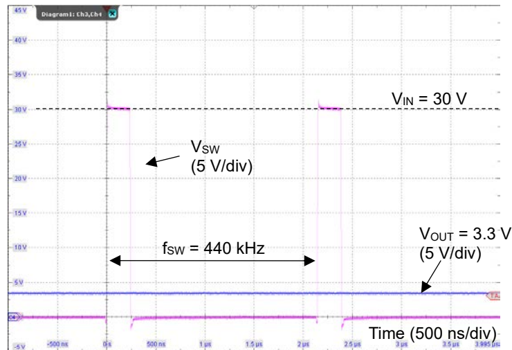
Figure 29. スイッチング波形 ( V_{IN} = 30 V, V_{OUT} = 3.3 V, I_{OUT} = 1.0 A, f_{SW} = 440 kHz)
