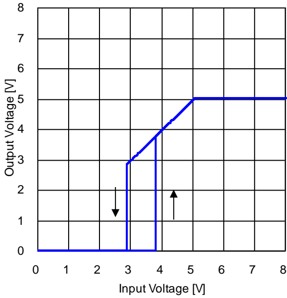
Figure 84. 出力電圧 vs 入力電圧 1 (R LOAD = 250 Ω)
