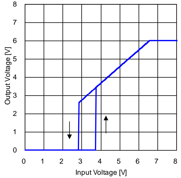
Figure 59. 出力電圧 vs 入力電圧 2 (R LOAD = 3 Ω)
