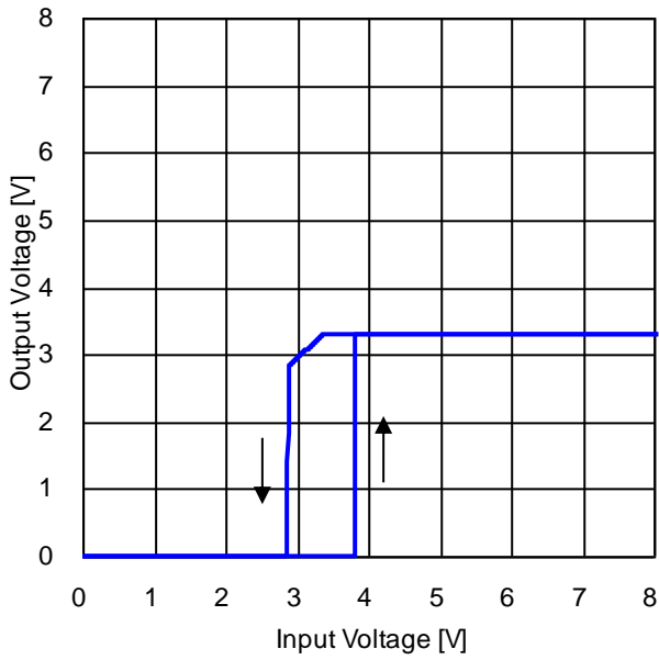
Figure 71. 出力電圧 vs 入力電圧 1 (R LOAD = 165 Ω)
