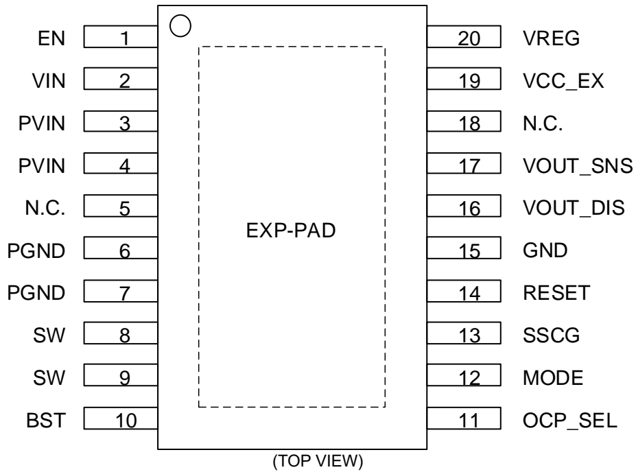
Figure 5. 端子配置図 (BD9P236EFV-C, BD9P256EFV-C)
