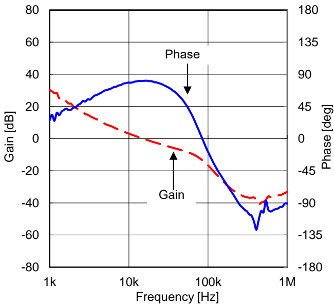
Figure 52. 周波数特性 ( V_{IN} = 12\text{ V} , I_{OUT} = 1.0\text{ A} )
