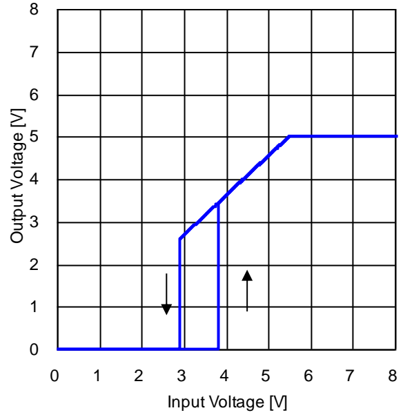
Figure 85. 出力電圧 vs 入力電圧 2 (R LOAD = 2.5 Ω)
