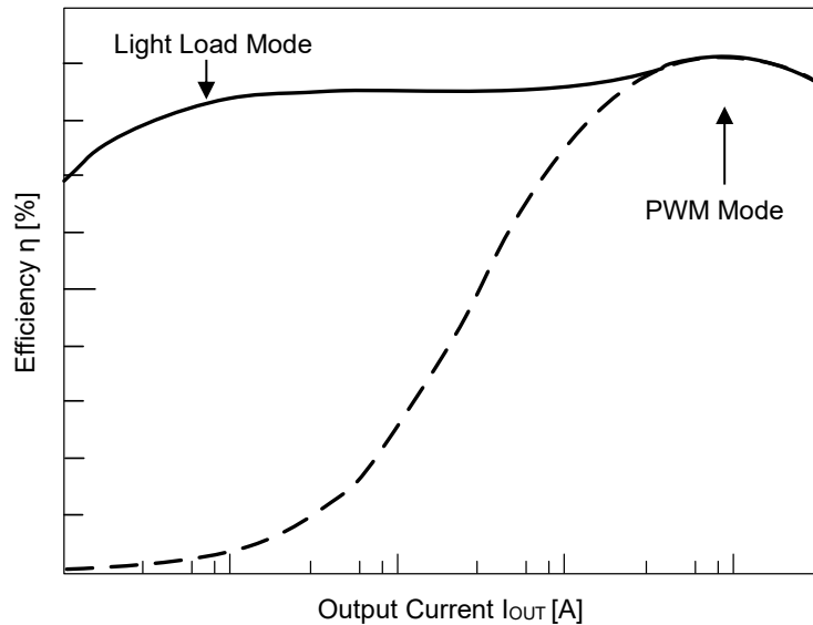
Figure 30. 効率 (Light Load Mode, PWM Mode)
