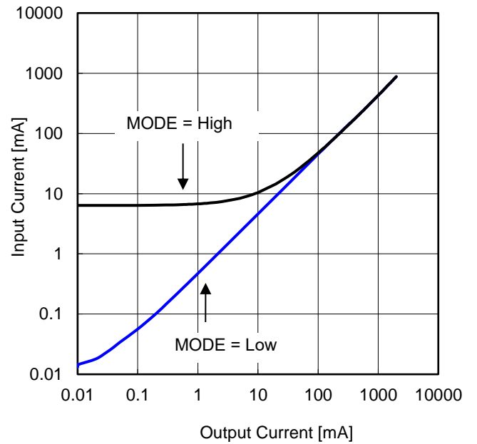
Figure 77. 入力電流 vs 負荷電流 ( V_{IN} = 12\text{ V} )
