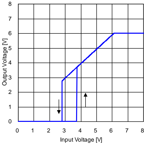
Figure 58. 出力電圧 vs 入力電圧 1 (R LOAD = 300 Ω)
