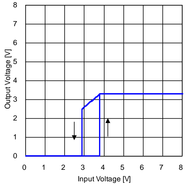
Figure 72. 出力電圧 vs 入力電圧 2 (R LOAD = 1.65 Ω)
