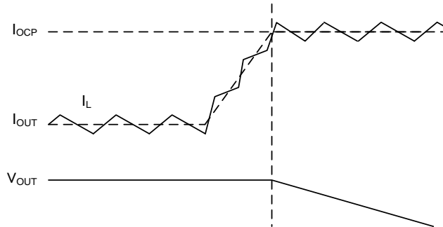
Figure 40. 過電流保護
