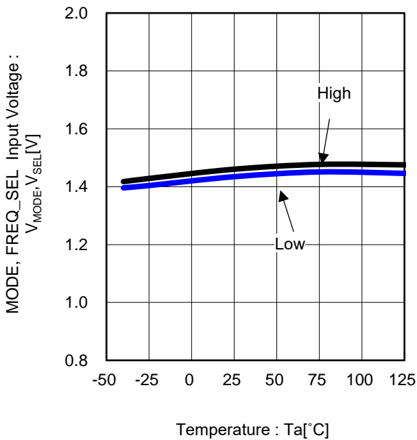
Figure 10. MODE, FREQ_SEL 入力電圧 vs 温度
