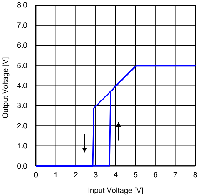
Figure 75. 出力電圧 vs 入力電圧 1 (R LOAD = 166 Ω)
