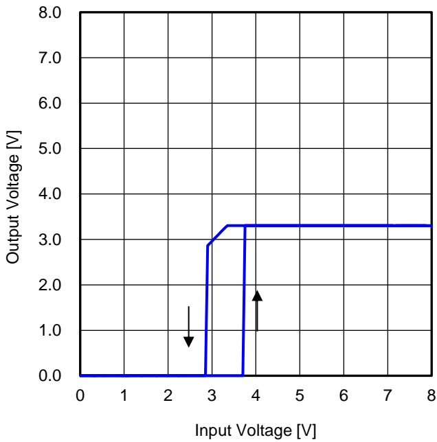
Figure 49. 出力電圧 vs 入力電圧 1 (R LOAD = 110 Ω)
