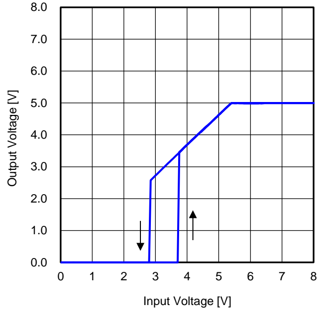
Figure 89. 出力電圧 vs 入力電圧 2 ( R_{LOAD} = 0.83\ \Omega )
