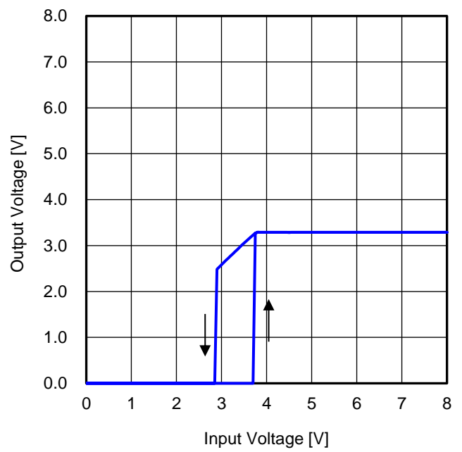
Figure 50. 出力電圧 vs 入力電圧 2 (R LOAD = 0.55 Ω)
