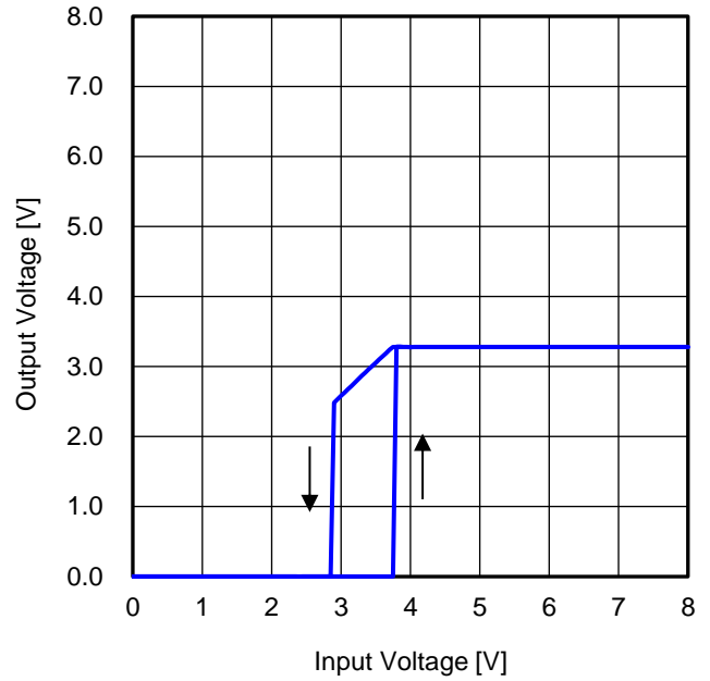
Figure 63. 出力電圧 vs 入力電圧 2 ( R_{LOAD} = 0.55 \Omega )
