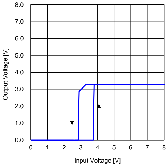
Figure 62. 出力電圧 vs 入力電圧 1 ( R_{LOAD} = 110 \Omega )
