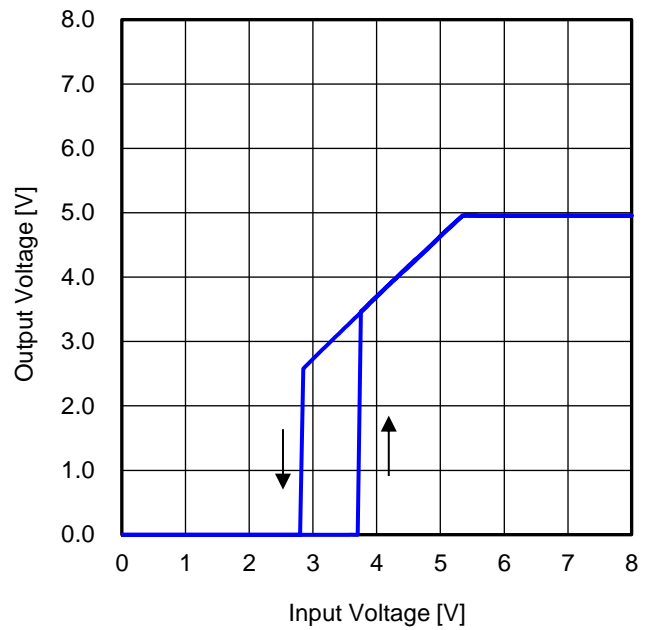
Figure 76. 出力電圧 vs 入力電圧 2 (R LOAD = 0.83 Ω)
