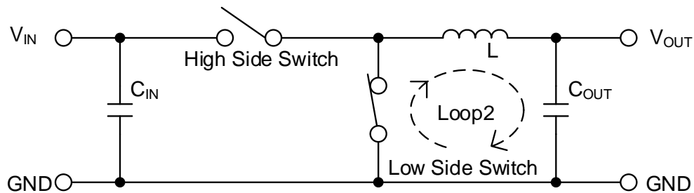
Figure 93 (b). High Side Switch : OFF、Low Side Switch : ON 時の電流経路
