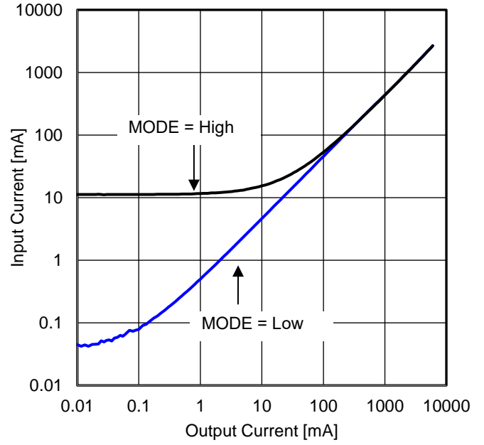
Figure 81. 入力電流 vs 負荷電流 ( V_{IN} = 12\text{ V} )
