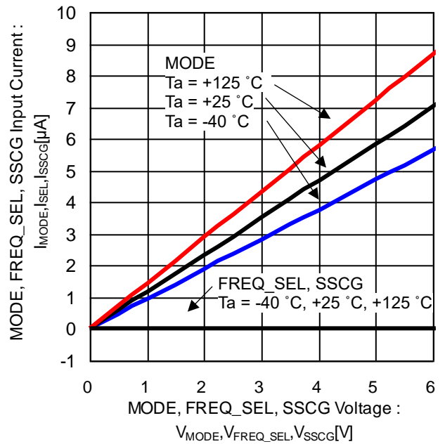
Figure 11. MODE, FREQ_SEL, SSCG 流入電流 vs MODE, FREQ_SEL, SSCG 電圧
