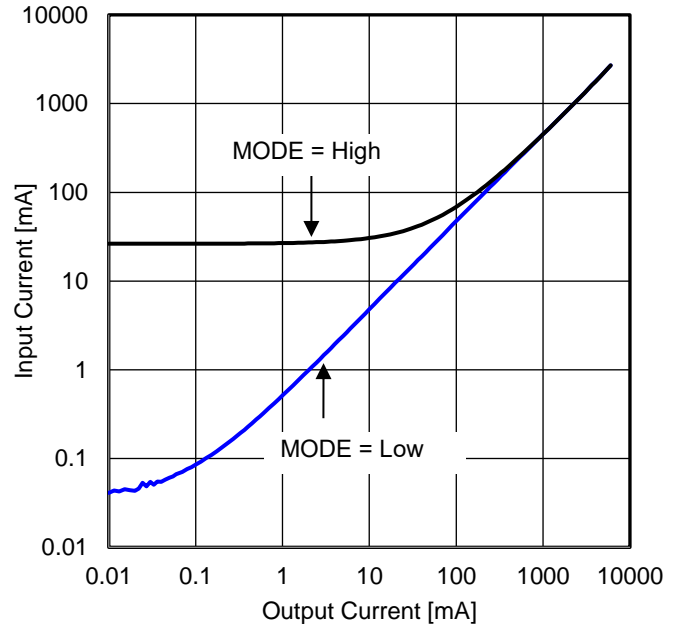
Figure 68. 入力電流 vs 負荷電流 ( V_{IN} = 12\text{ V} )
