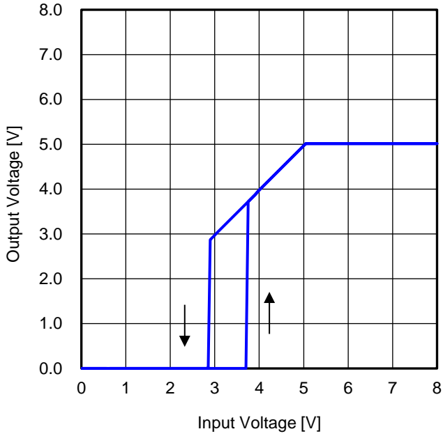
Figure 88. 出力電圧 vs 入力電圧 1 ( R_{LOAD} = 166\ \Omega )
