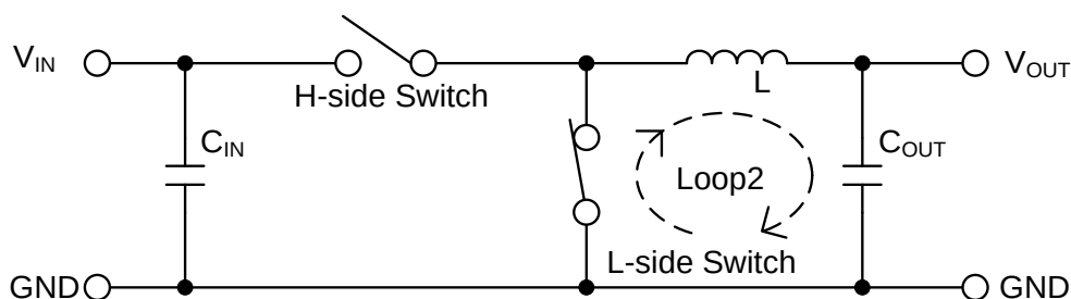
Figure 54-b. H-side Switch: OFF、L-side Switch: ON 時の電流経路
