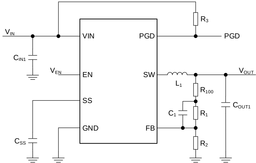
Figure 29. Reference Circuit 1
