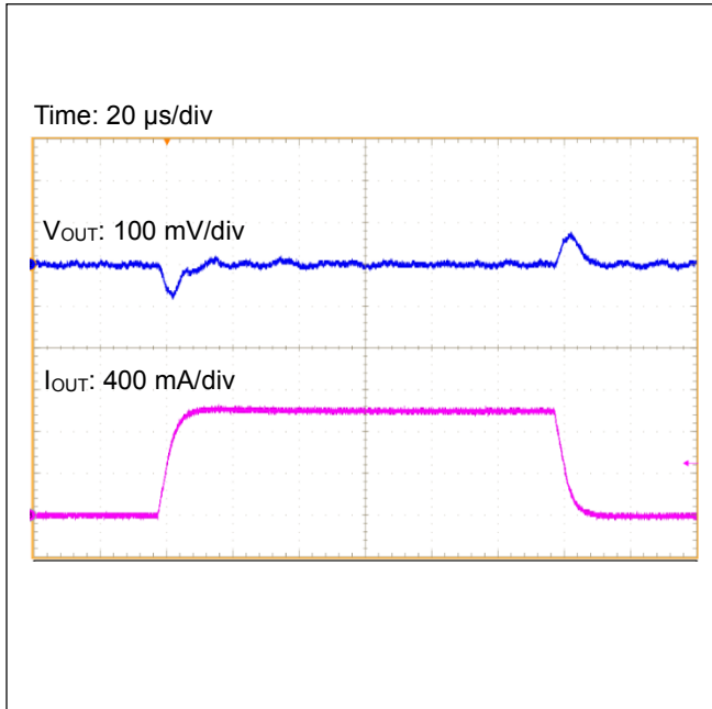
Figure 32. 負荷応答 ( I_{OUT} = 0\text{ A} \leftrightarrow 1\text{ A} )
