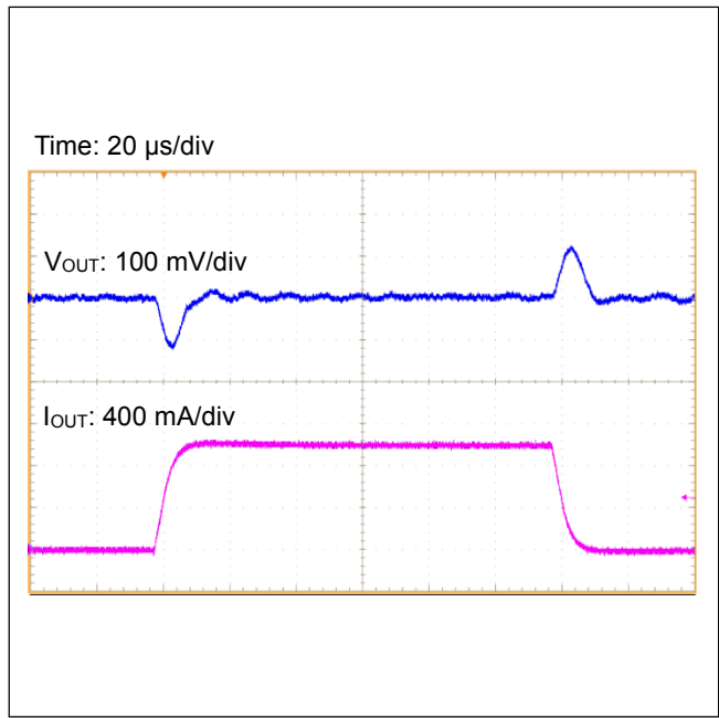
Figure 47. 負荷応答 ( I_{OUT} = 0\text{ A} \leftrightarrow 1\text{ A} )
