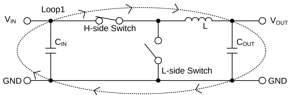
Figure 54-a. H-side Switch: ON、L-side Switch: OFF 時の電流経路
