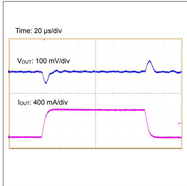
Figure 42. 負荷応答 ( I_{OUT} = 0\text{ A} \leftrightarrow 1\text{ A} )
