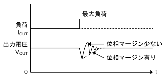
Figure 39. 負荷応答
