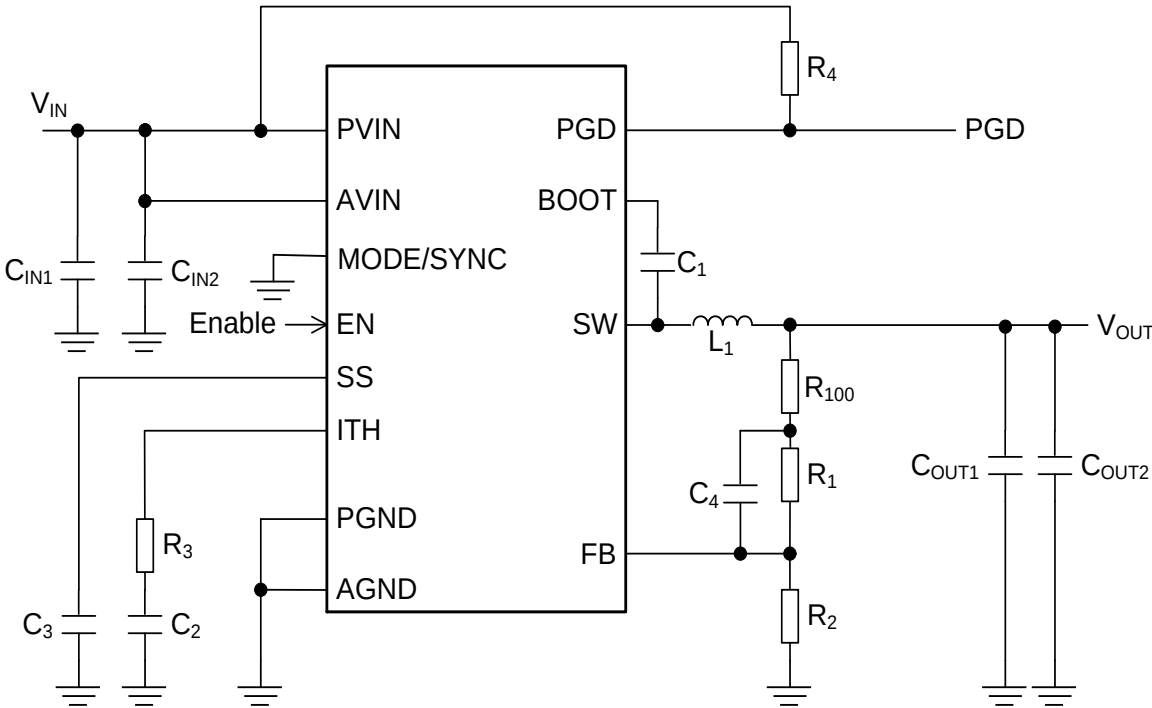
Figure 61. Reference Circuit 5
