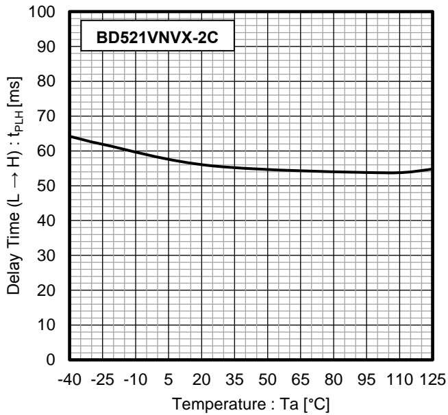
Figure 11. Delay Time (L → H) vs Temperature ( C_{CT} = 10 nF)
