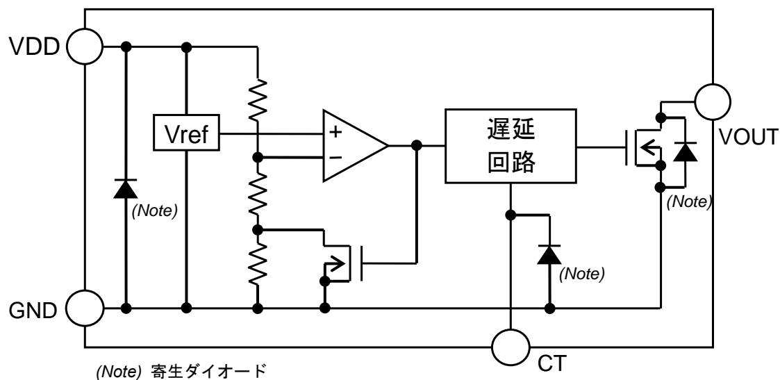
Figure 2. BD521VNVX-2C
