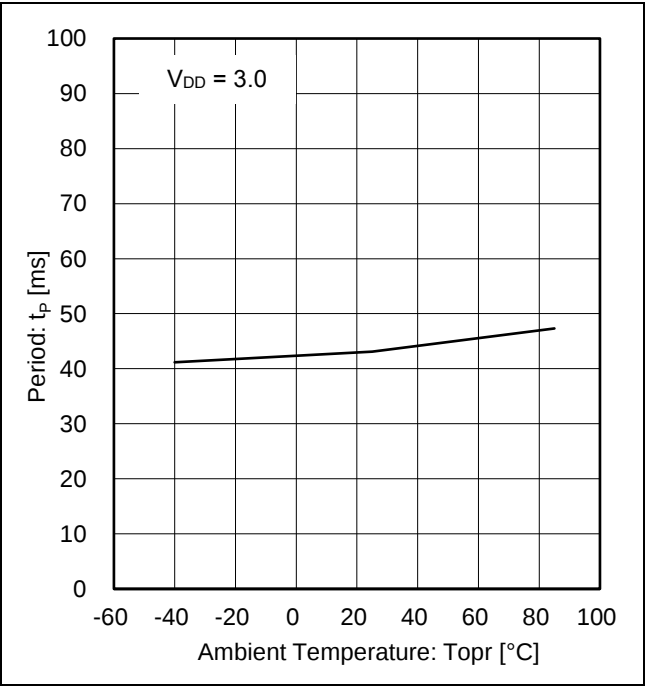
Figure 7. Period vs Ambient Temperature
