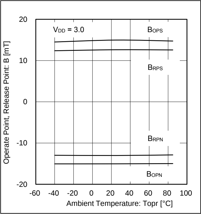
Figure 5. Operate Point, Release Point vs Ambient Temperature
