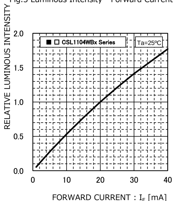
Fig.3 Luminous Intensity - Forward Current
