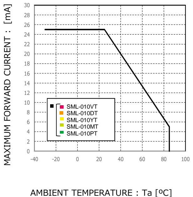
Fig.4 Derating
