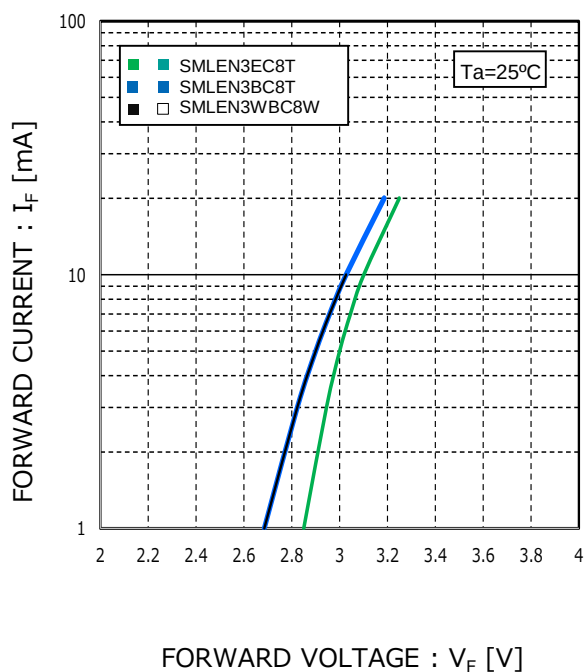
Fig.1 Forward Current - Forward Voltages
