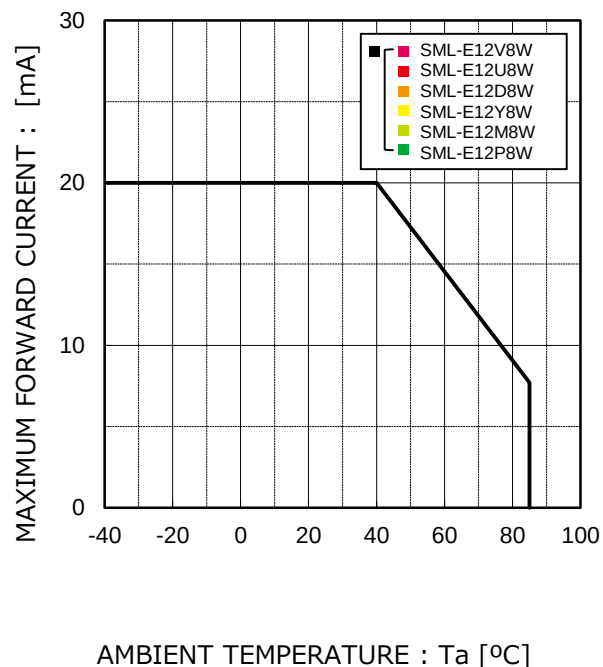
Fig.4 Derating
