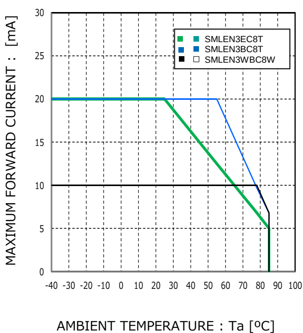
Fig.4 Derating
