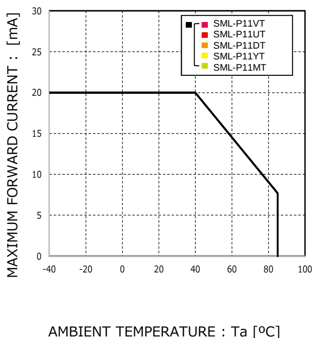
Fig.4 Derating
