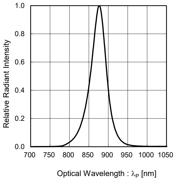
Fig.5 Spectral data
