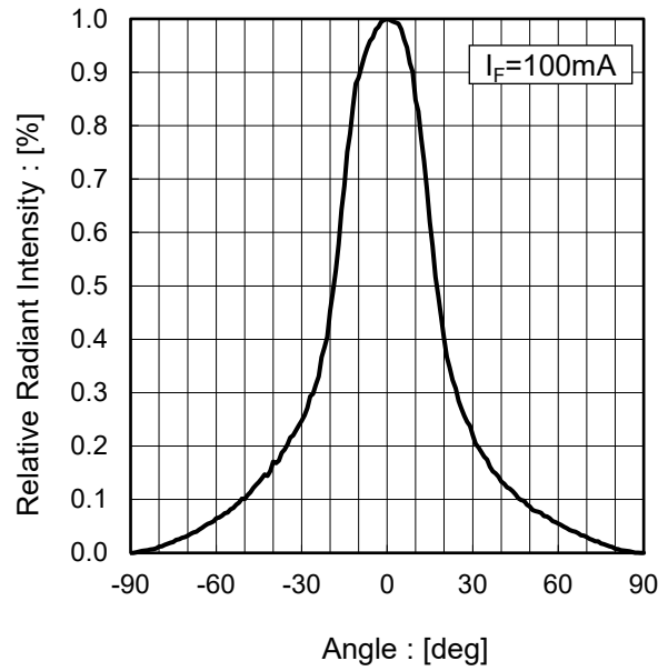
Fig.6 Radiant intensity
