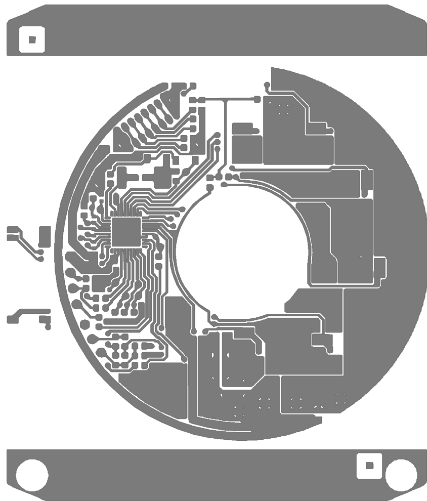
Top_Layer
