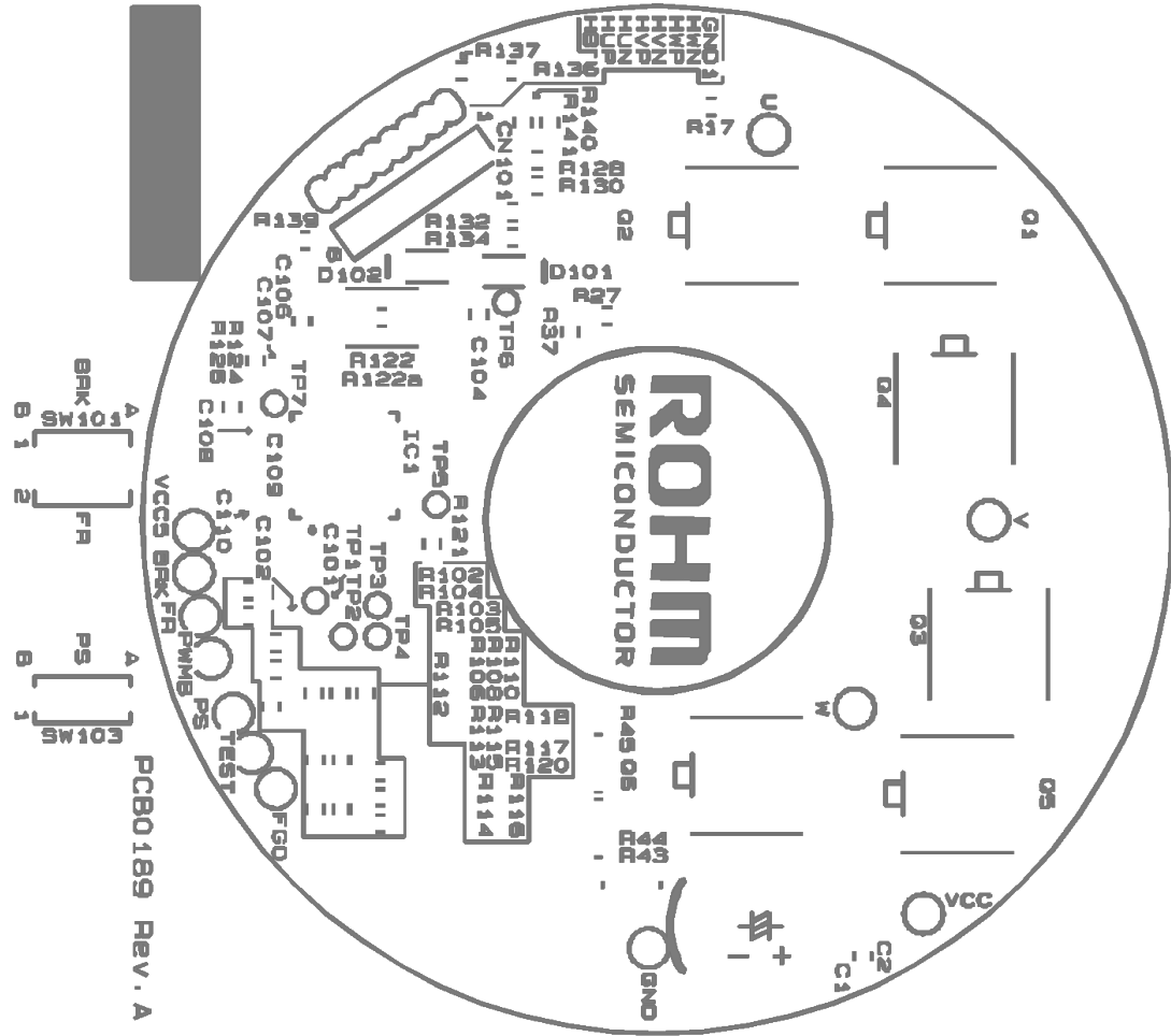
Top_Silk
