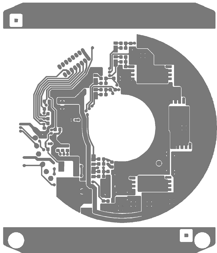
Bottom_Layer
