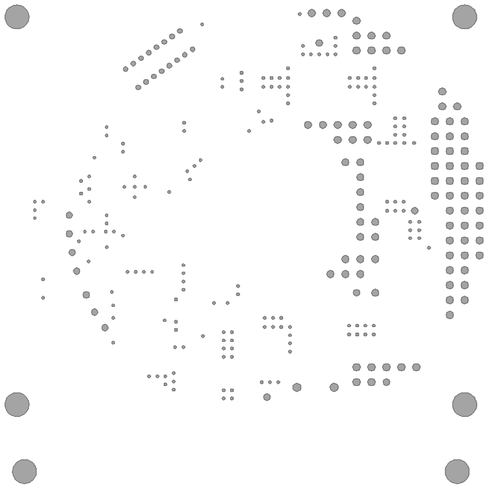
Drill_PTH
