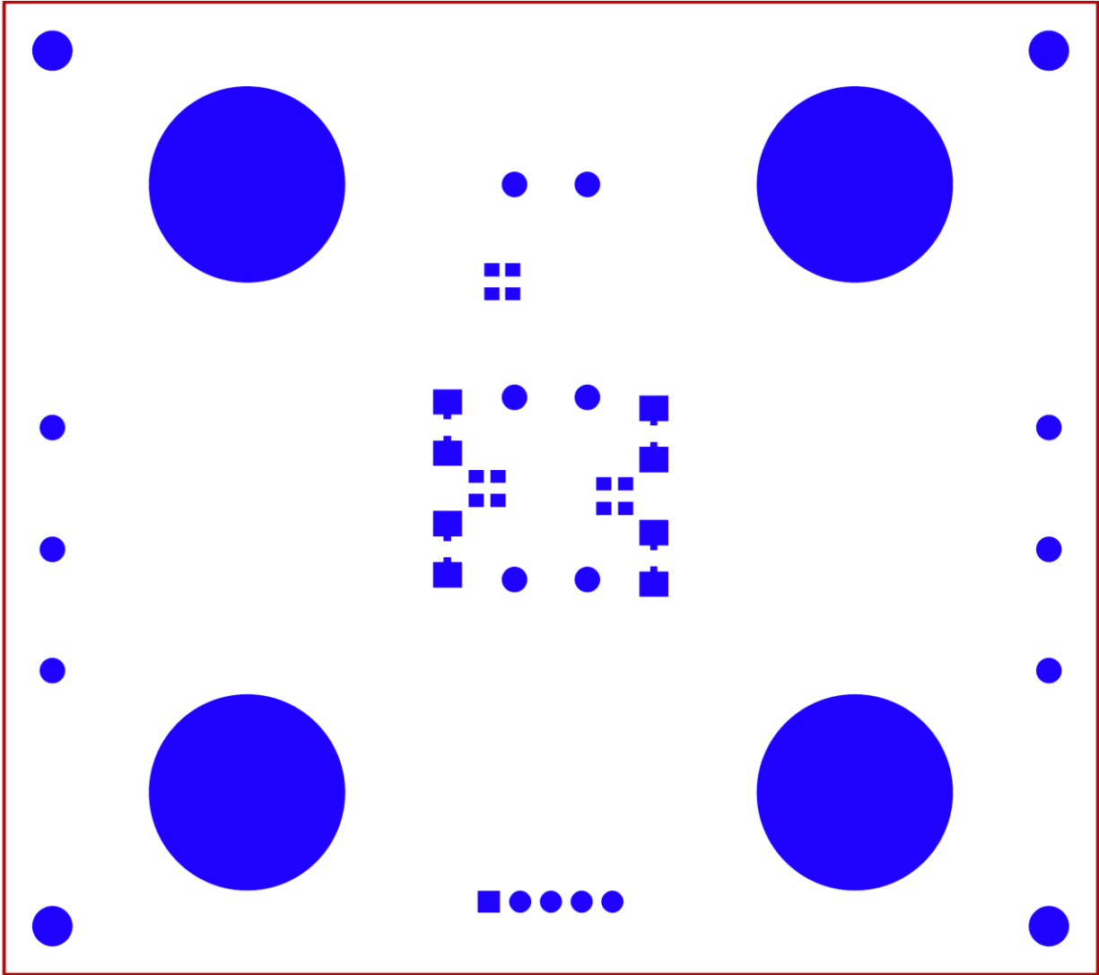
Top View Bottom Solder Mask
