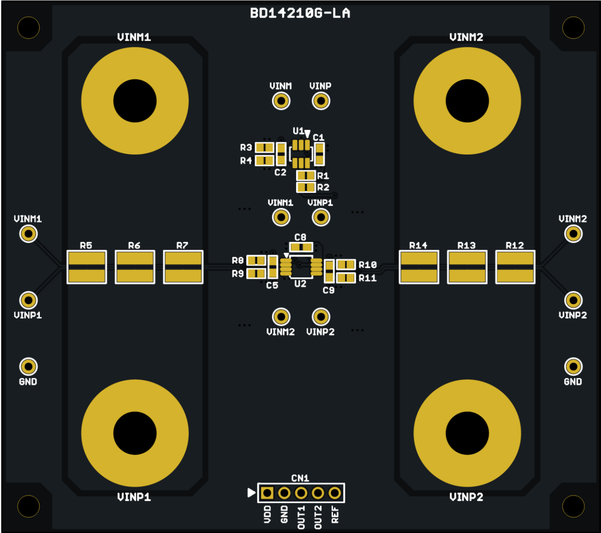
Top View Top PCB Image
