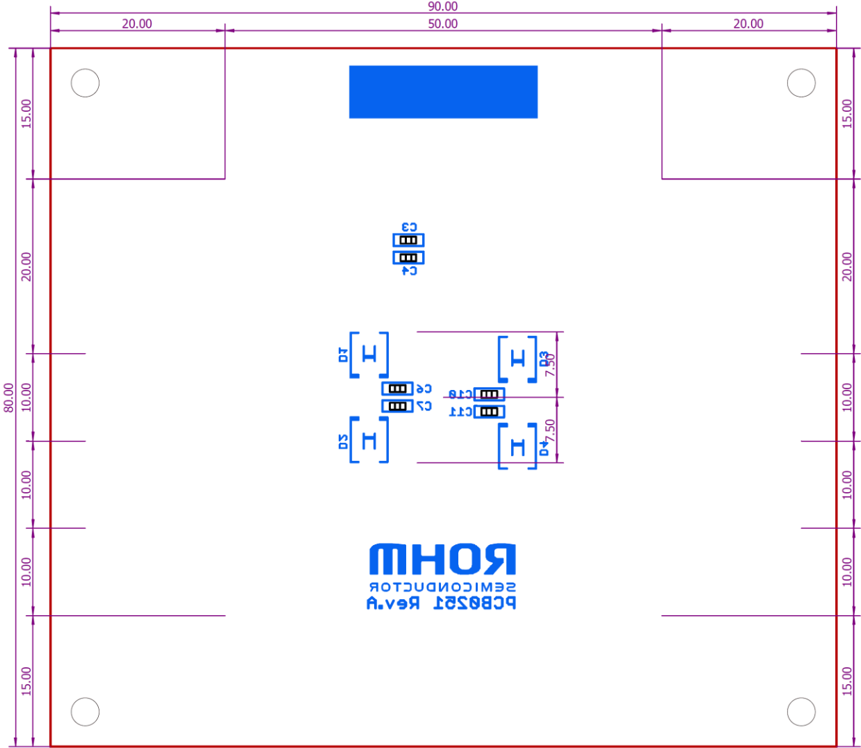
Top View Bottom Silkscreen Overlay
