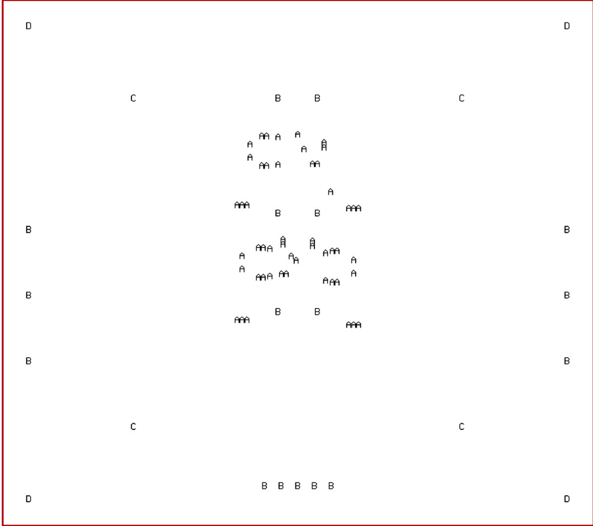
Top View Drill Drawing
