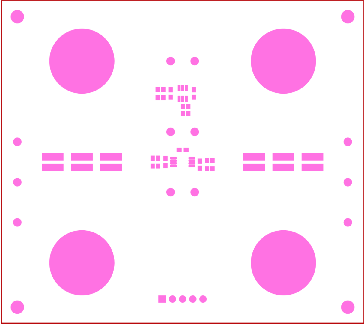
Top View Top Solder Mask
