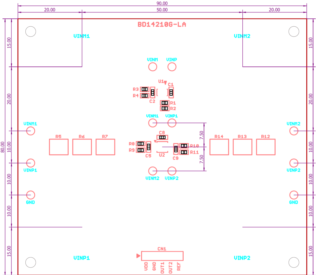
Top View Top Silkscreen Overlay
