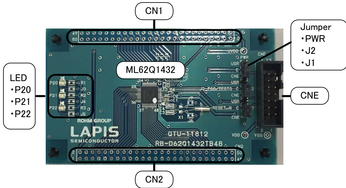
Fig.1 ML62Q1432 Reference Board Outline Drawing
