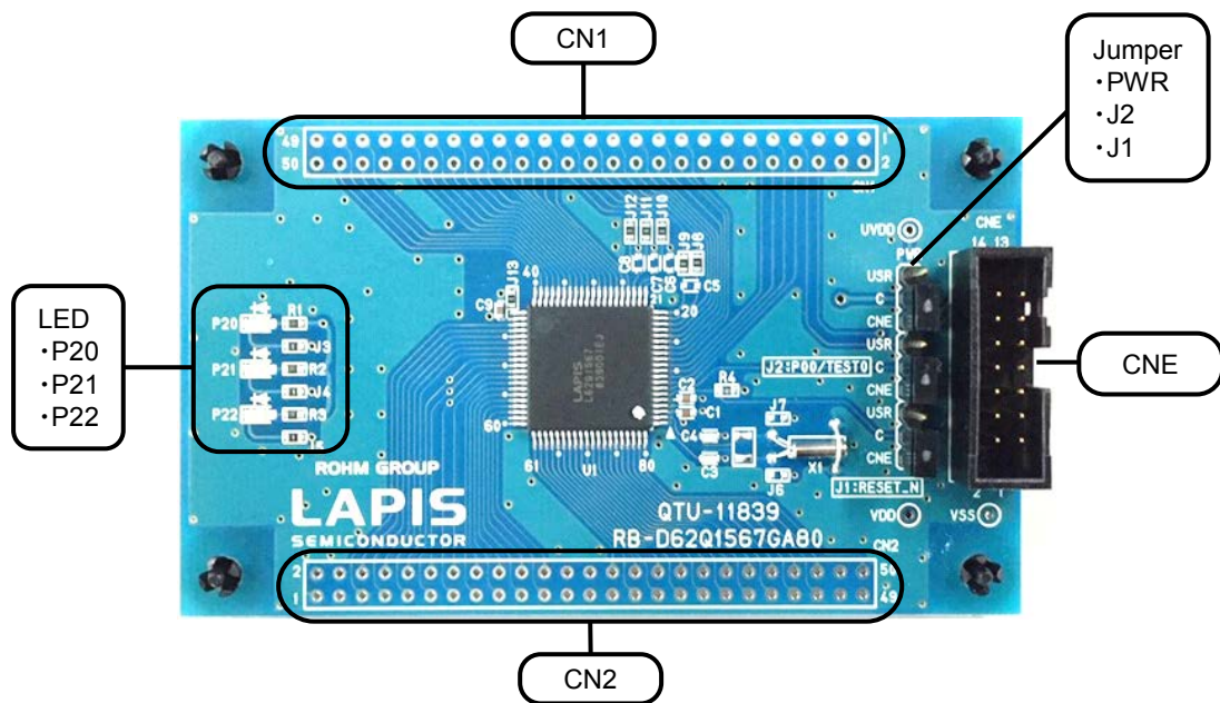
Fig. 1 ML62Q1567 Reference Board Outline Diagram
