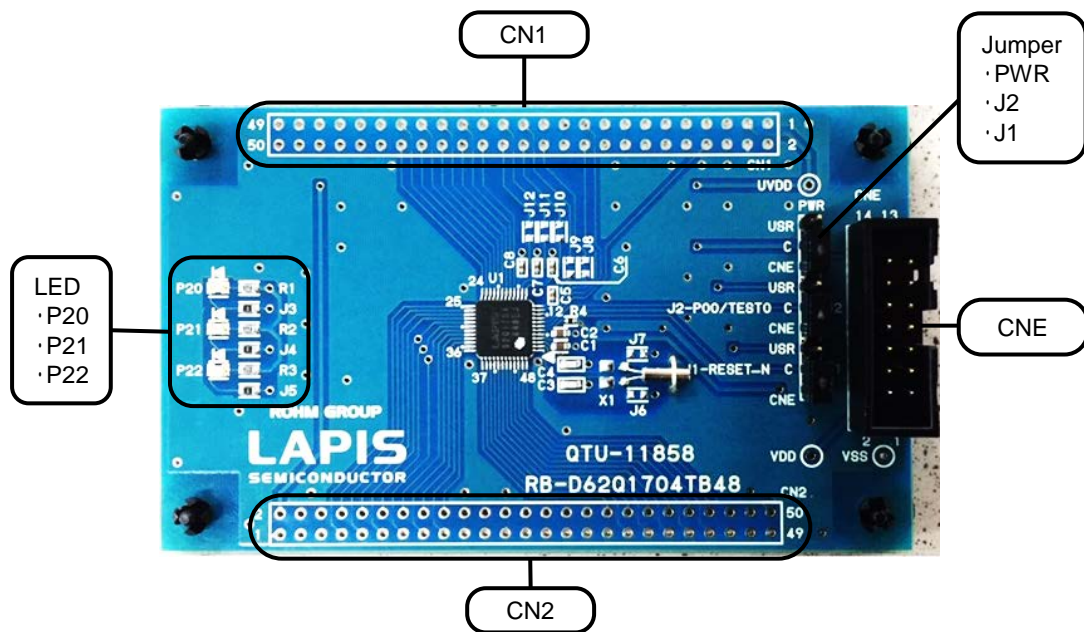
Fig. 1 ML62Q1704 Reference Board Outline Diagram
