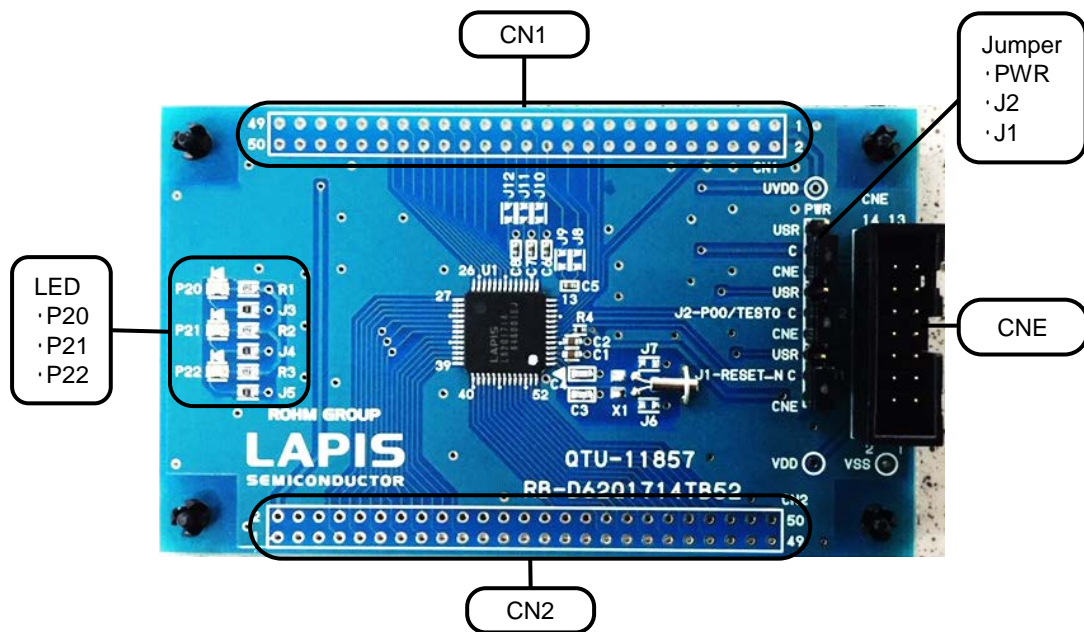
Fig. 1 ML62Q1714 Reference Board Outline Diagram
