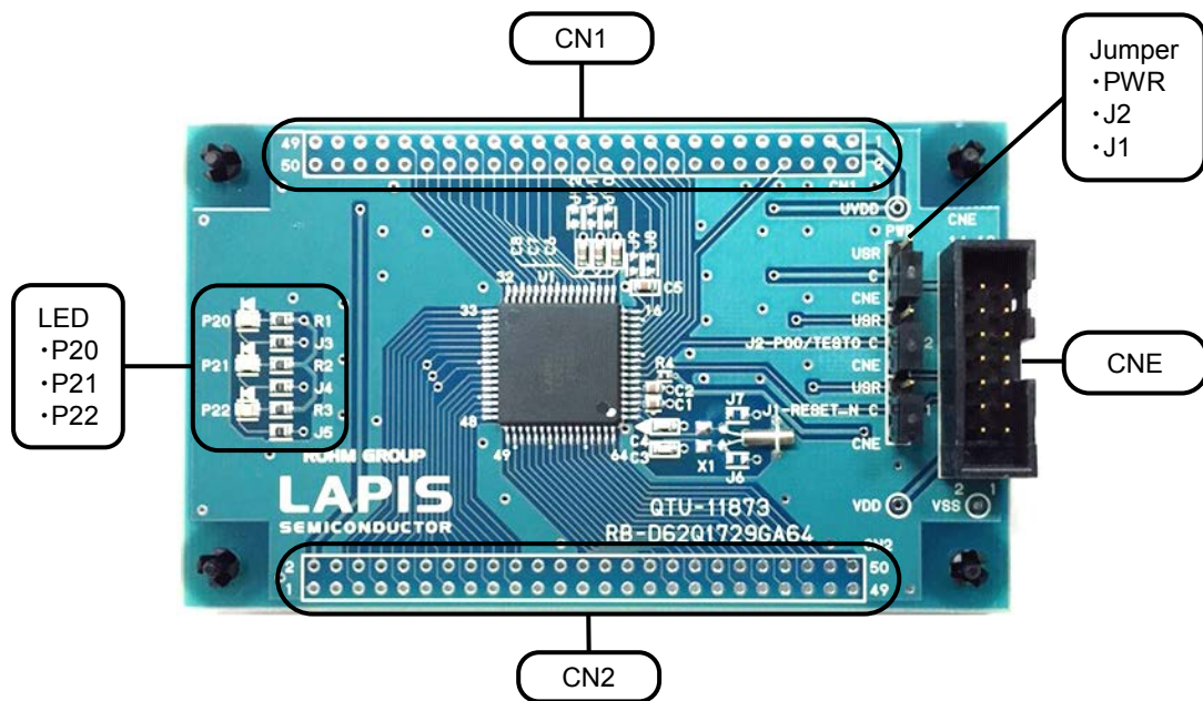
Fig. 1 ML62Q1729 Reference Board Outline Diagram
