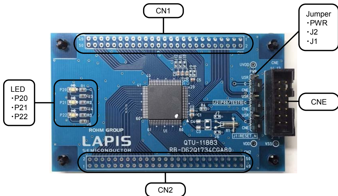
Fig. 1 ML62Q1734C Reference Board Outline Diagram
