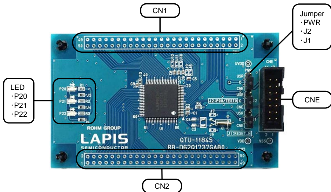
Fig. 1 ML62Q1737 Reference Board Outline Diagram
