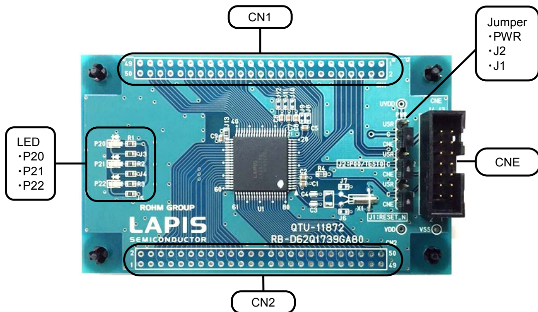
Fig. 1 ML62Q1739 Reference Board Outline Diagram
