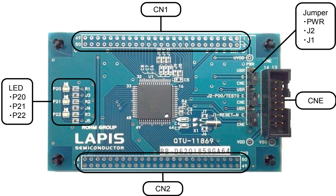
Fig. 1 ML62Q1859 Reference Board Outline Diagram
