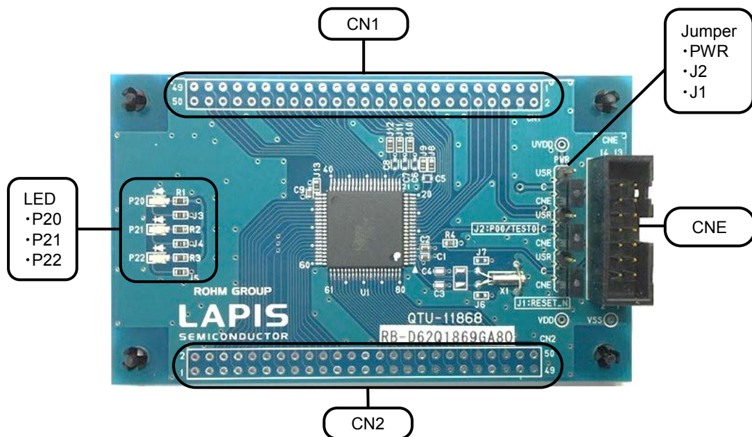
Fig. 1 ML62Q1869 Reference Board Outline Diagram
