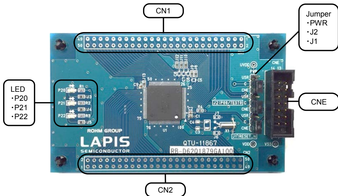
Fig. 1 ML62Q1879 Reference Board Outline Diagram
