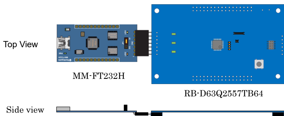
Fig. 7. Example of connection between SPI connection through hole (CN3) and MM-FT232H, MM-FT232HC
